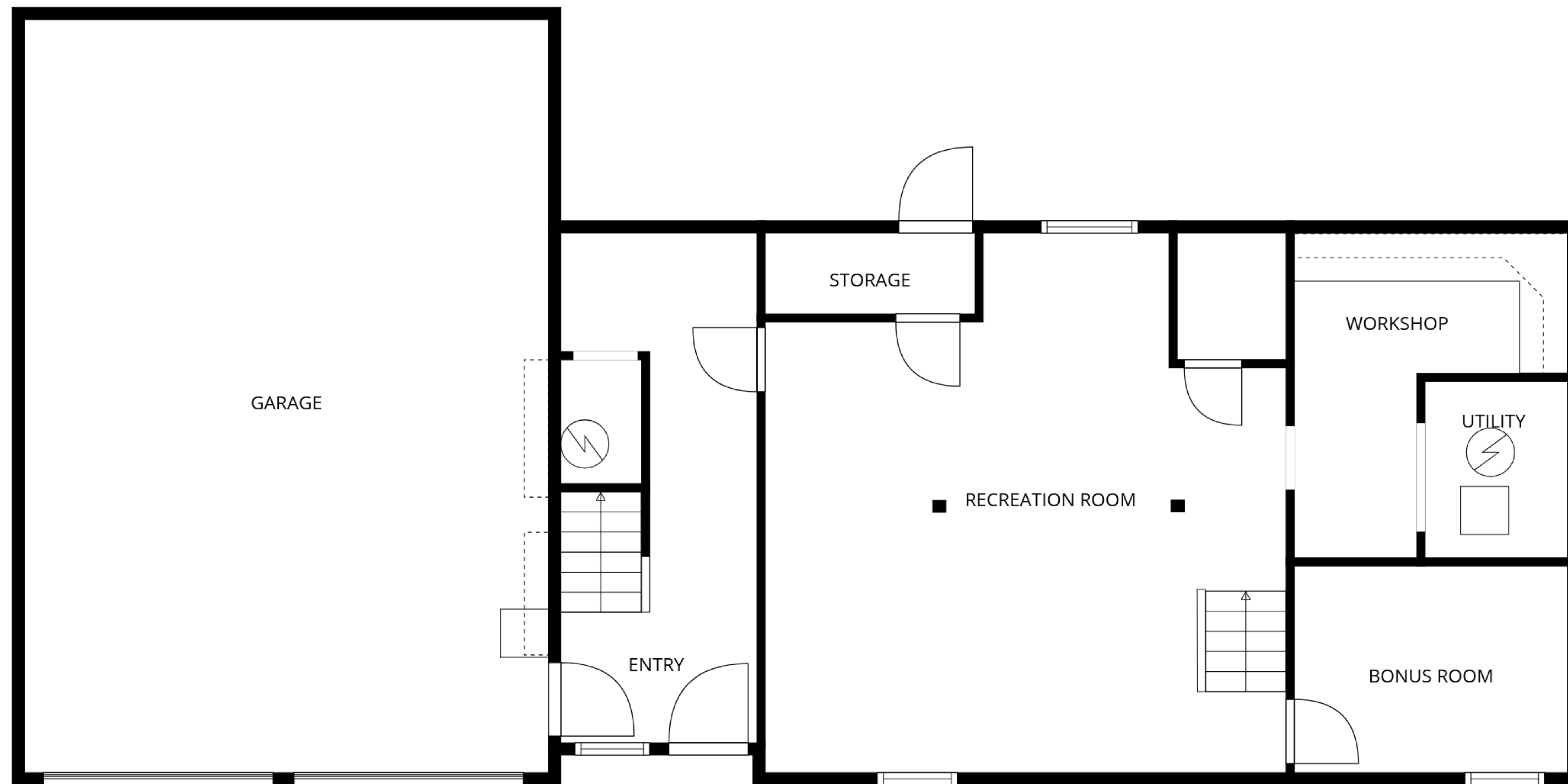
FLOOR 1
