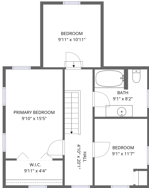
2nd floor
