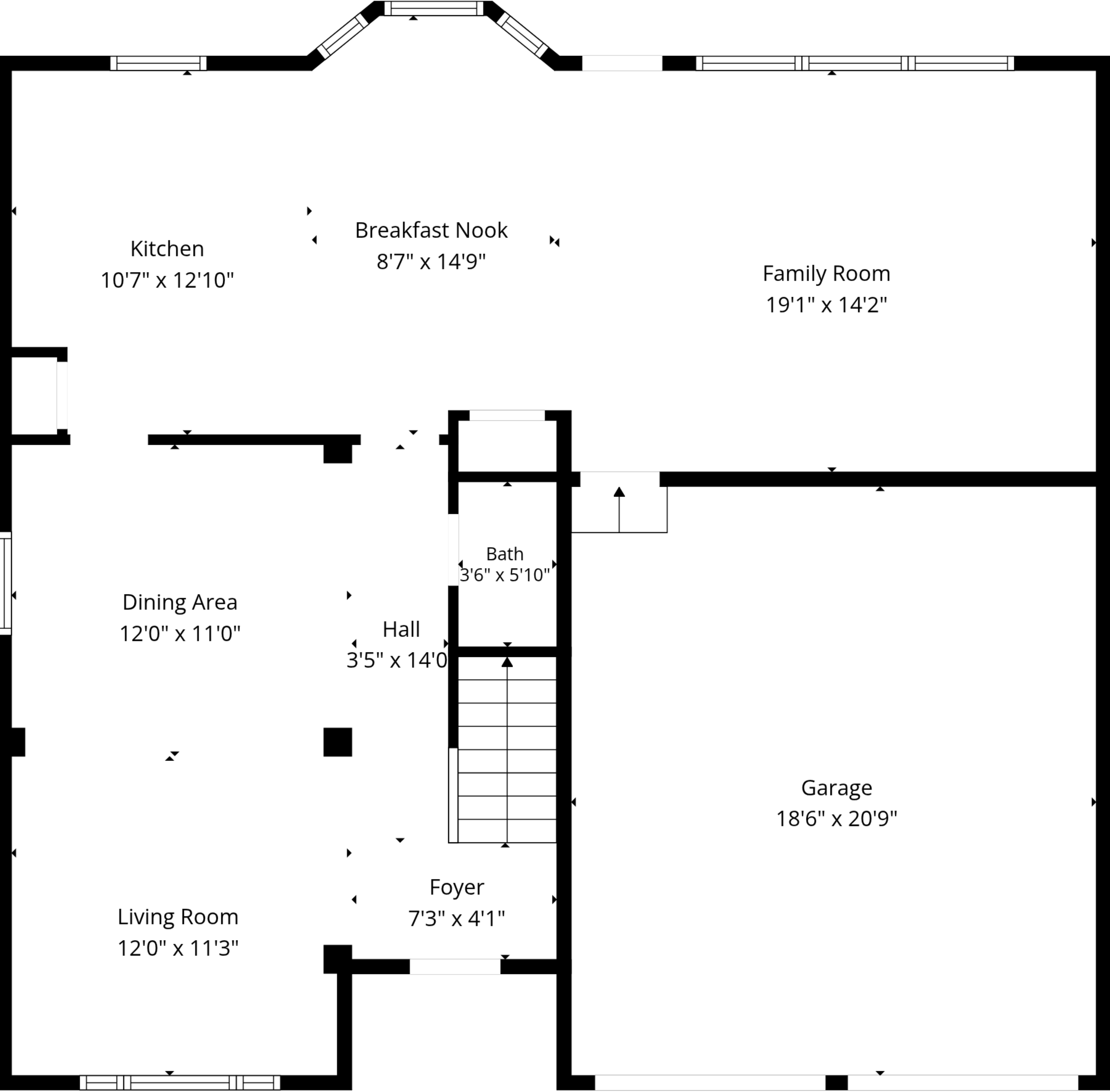
1st Floor
