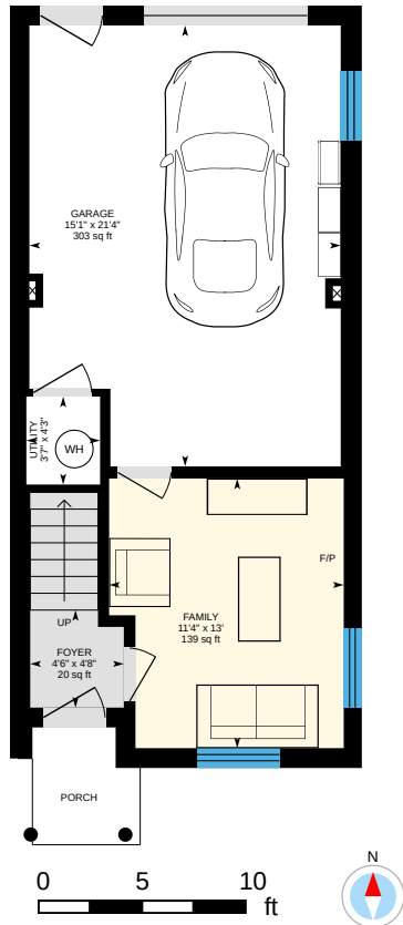
Entry Level (8ft) Exterior Area 233.96 sq ft
