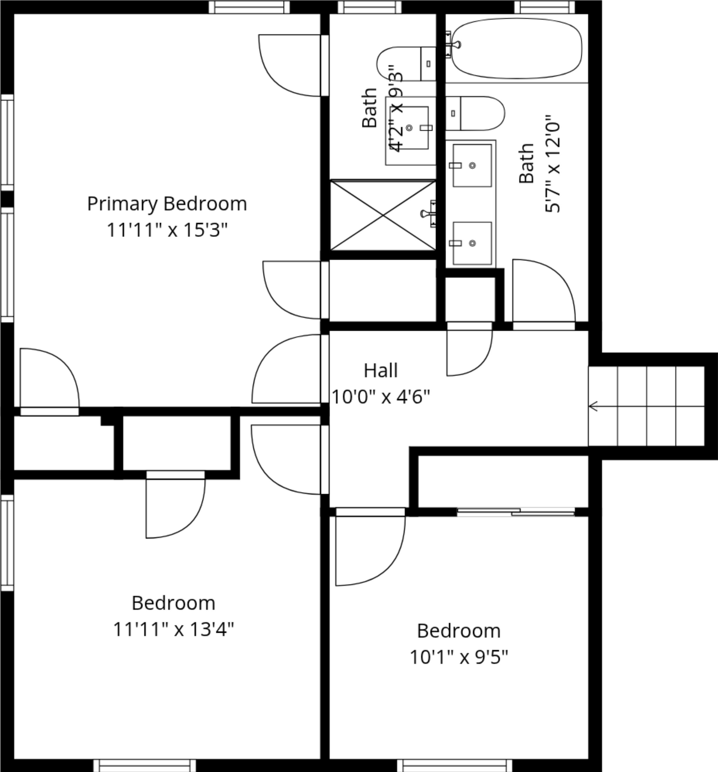
Floor 4
