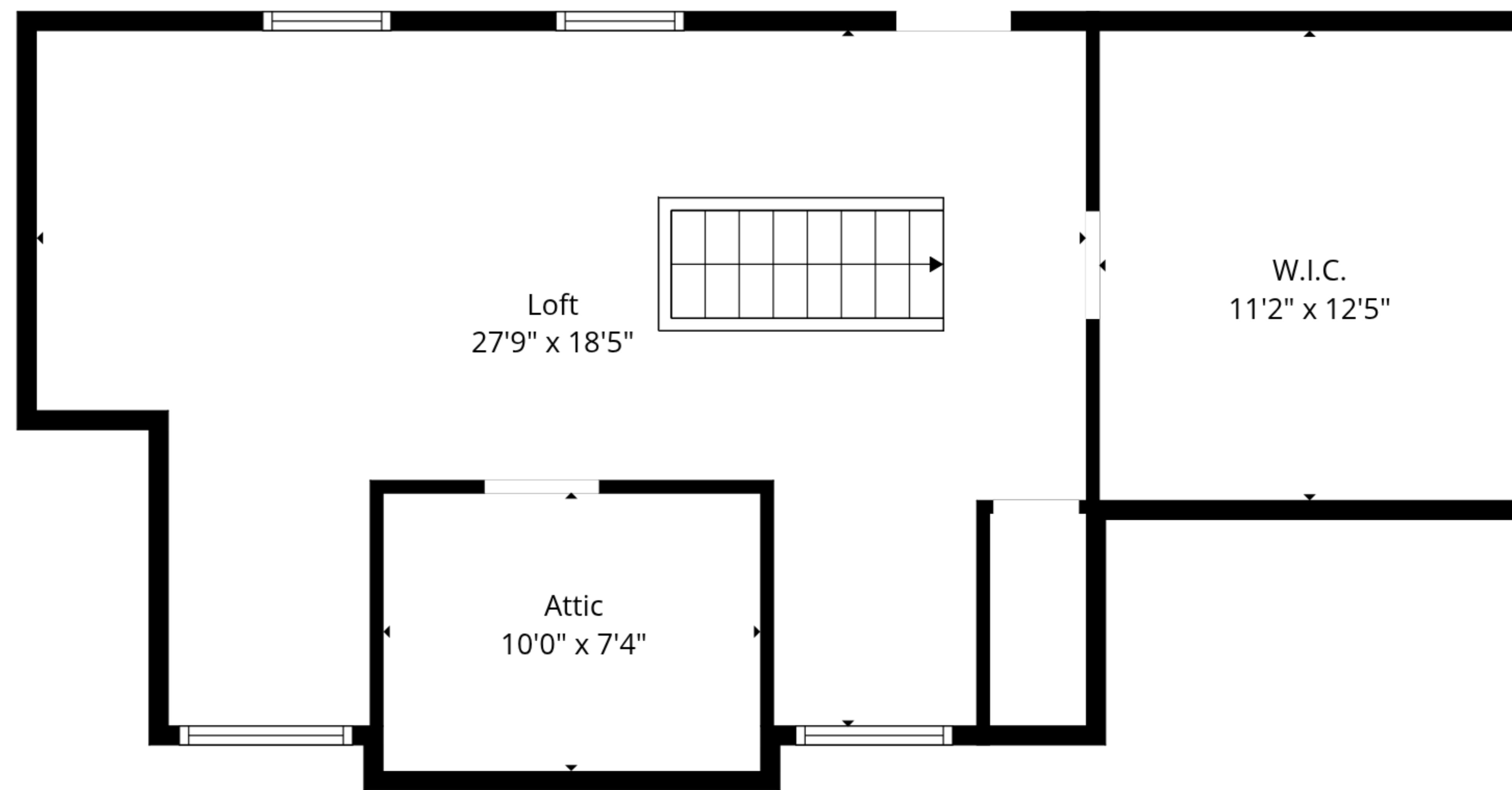
2nd Floor
