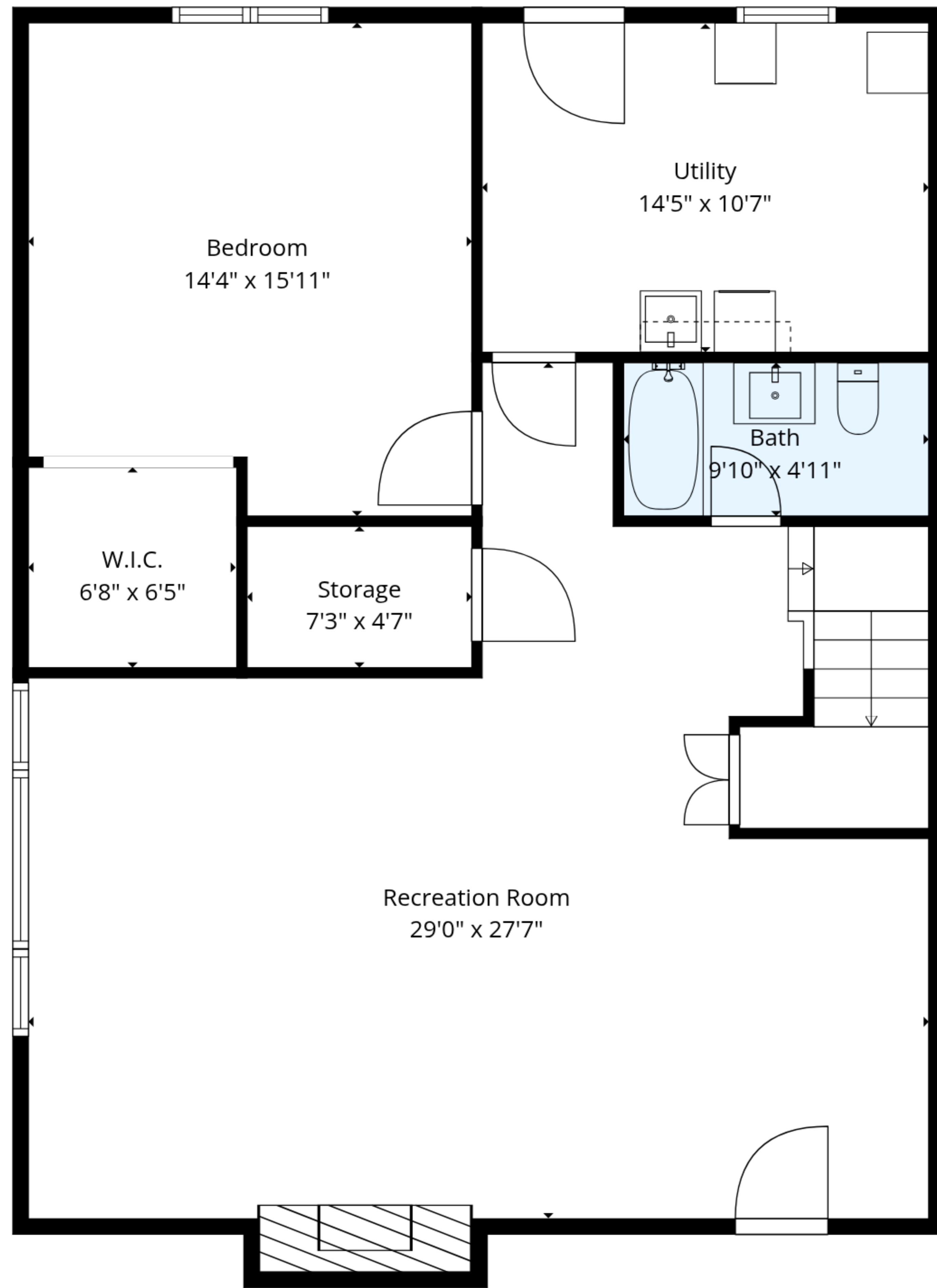
Basement
