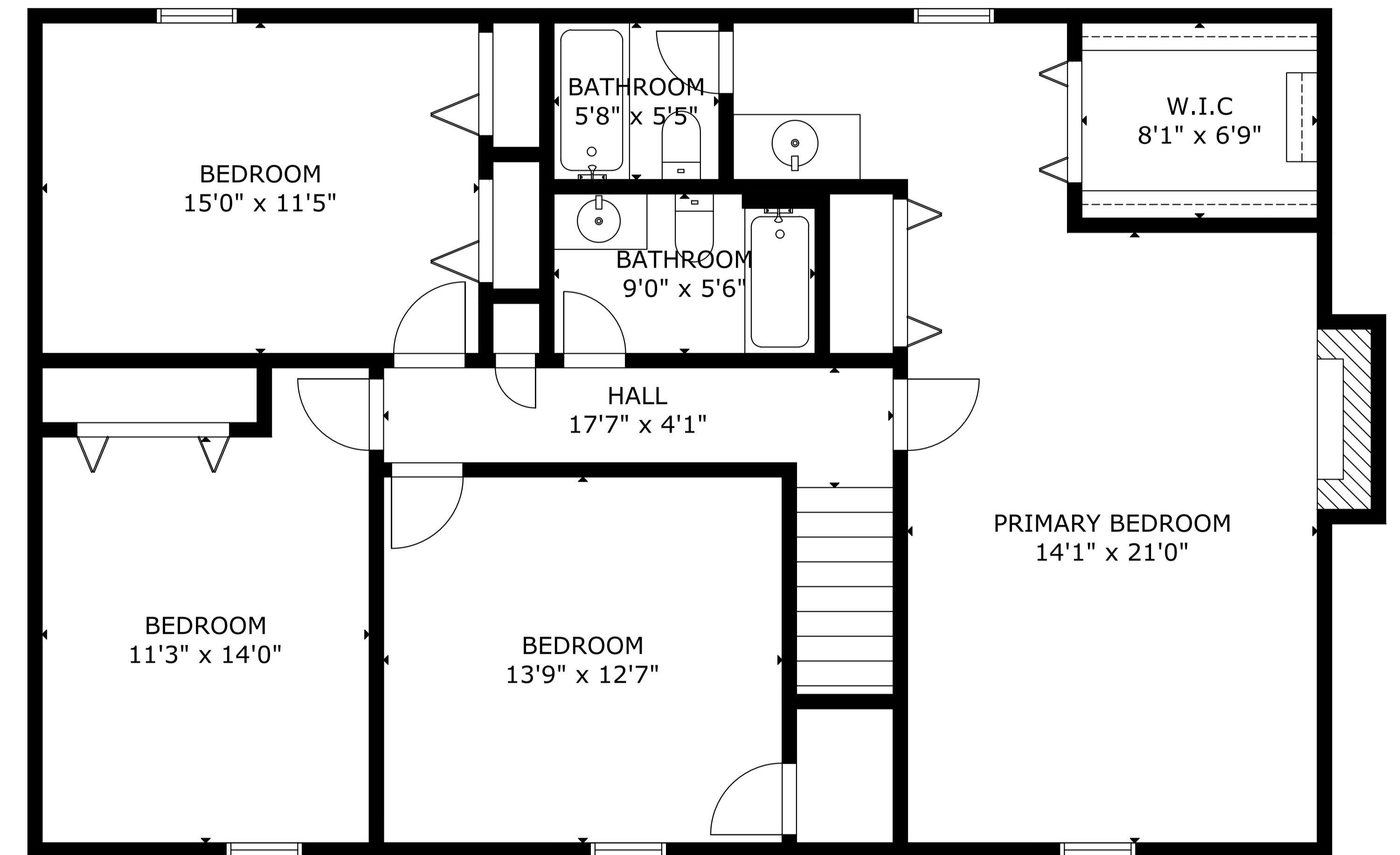
UPPER LEVEL 1
