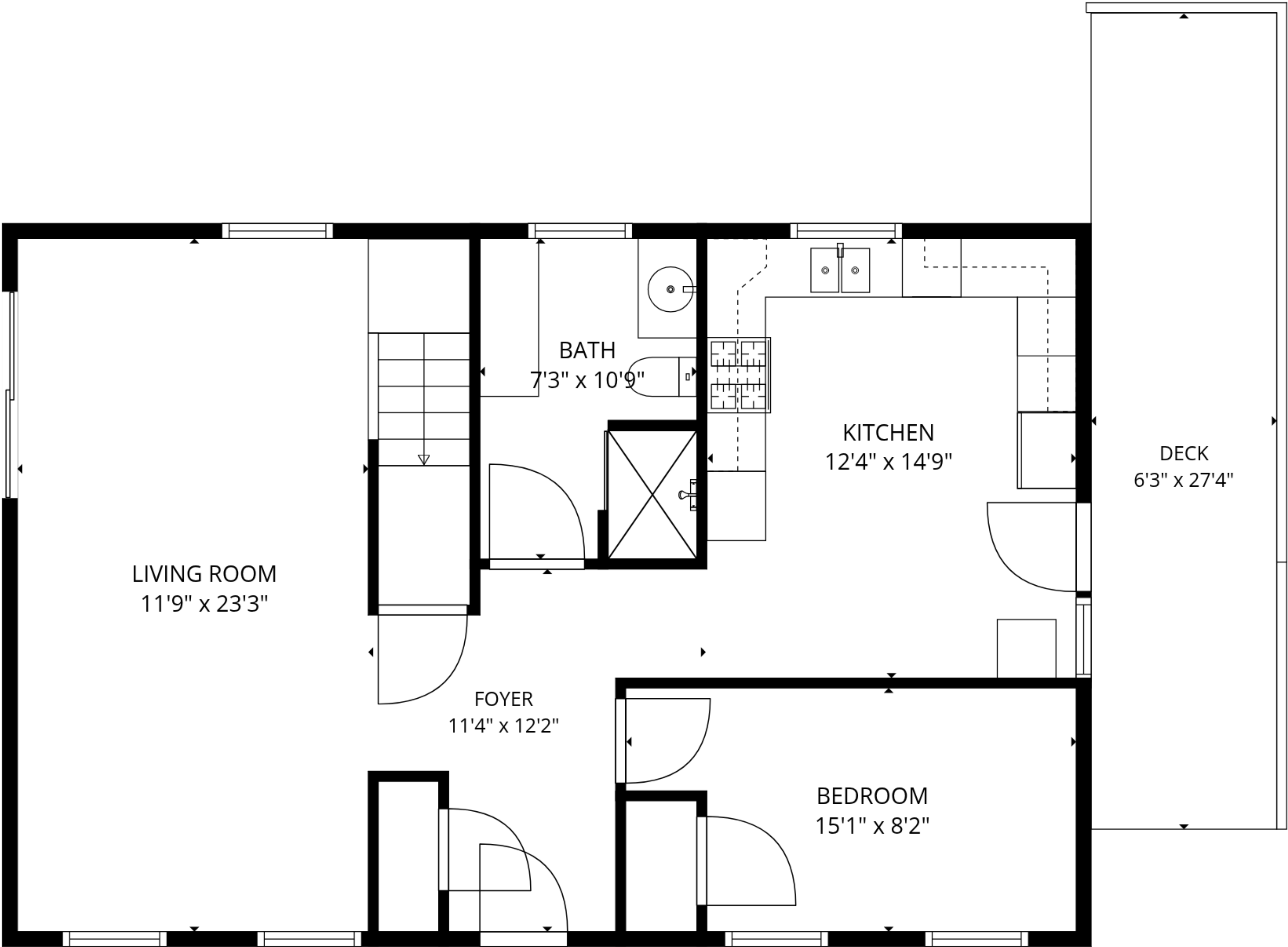
2nd floor
