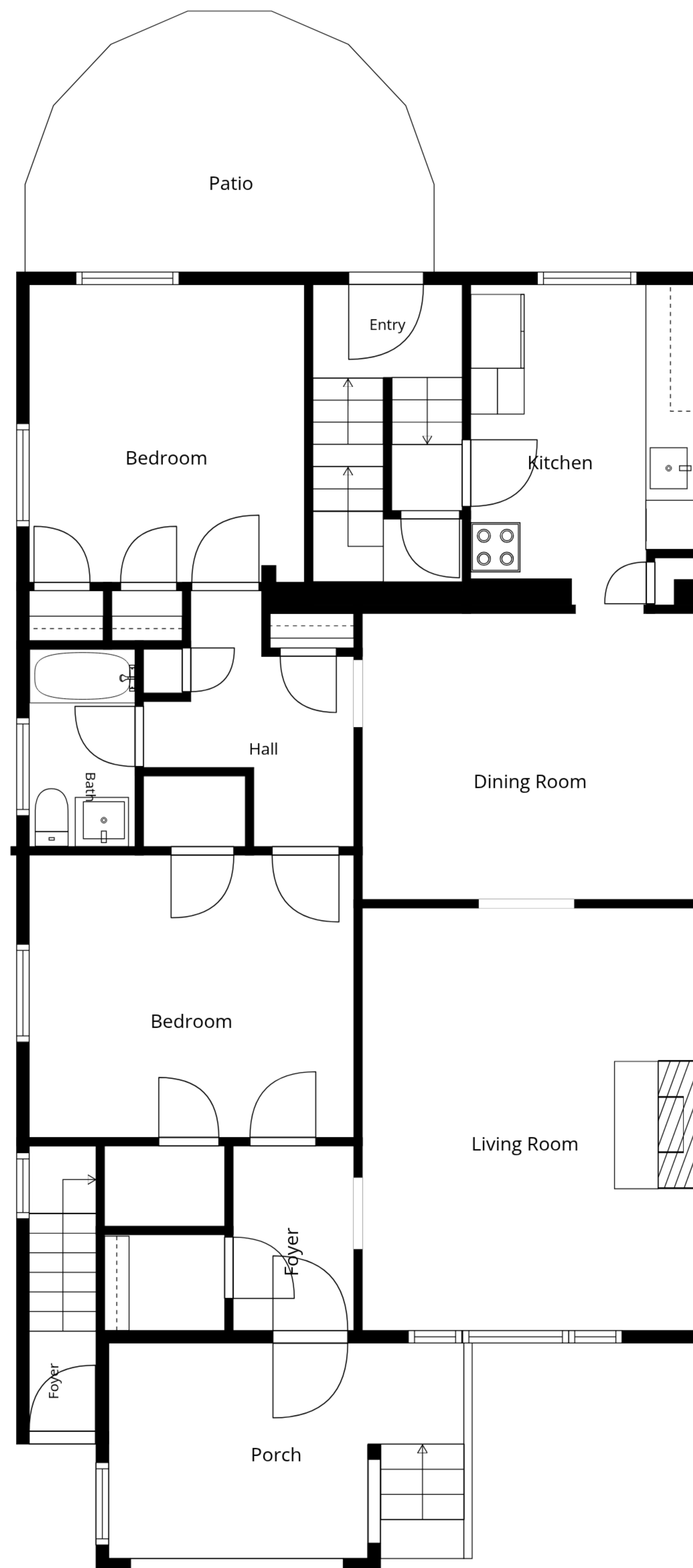
1st Floor
