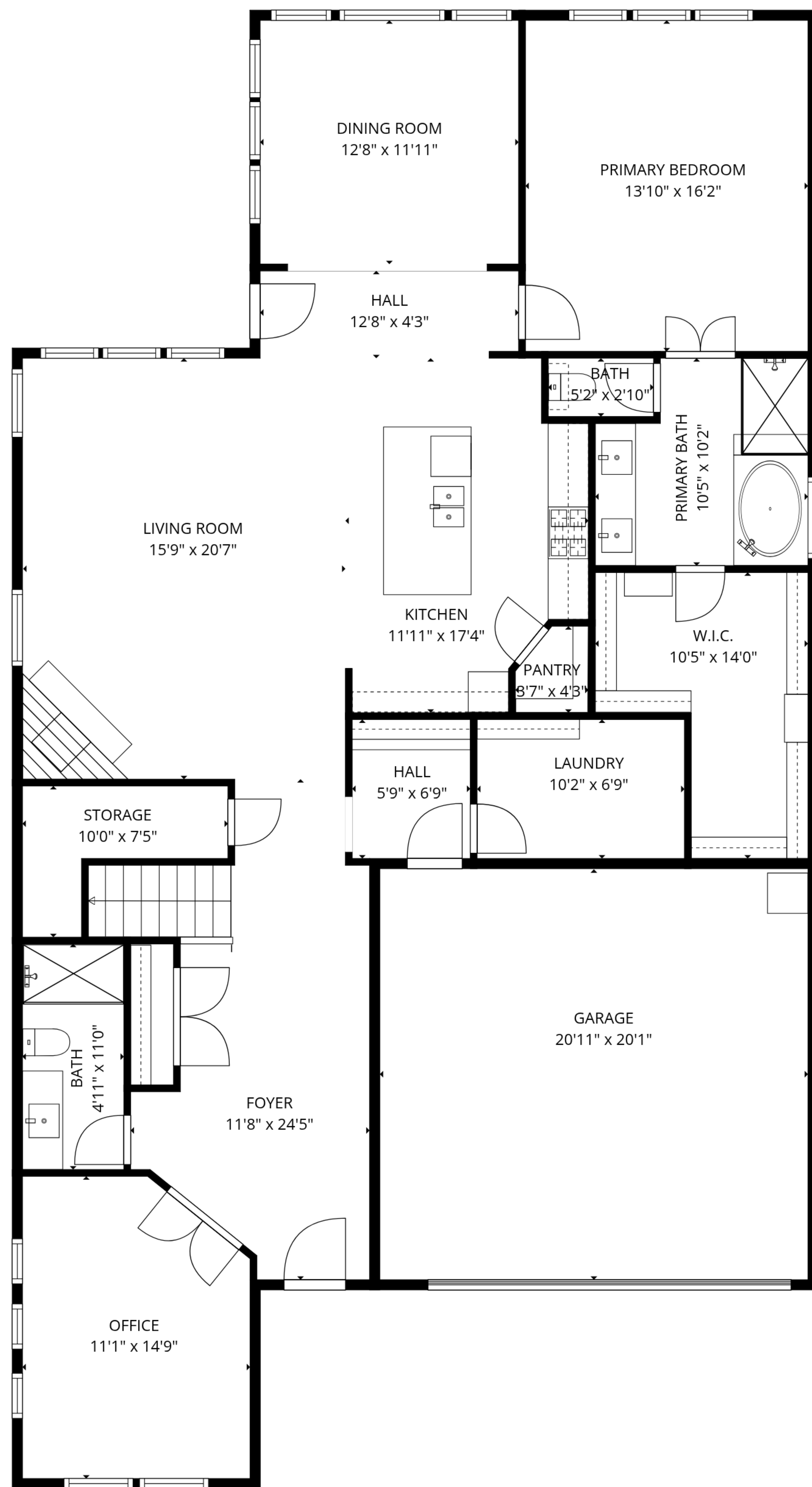
FLOOR 1
