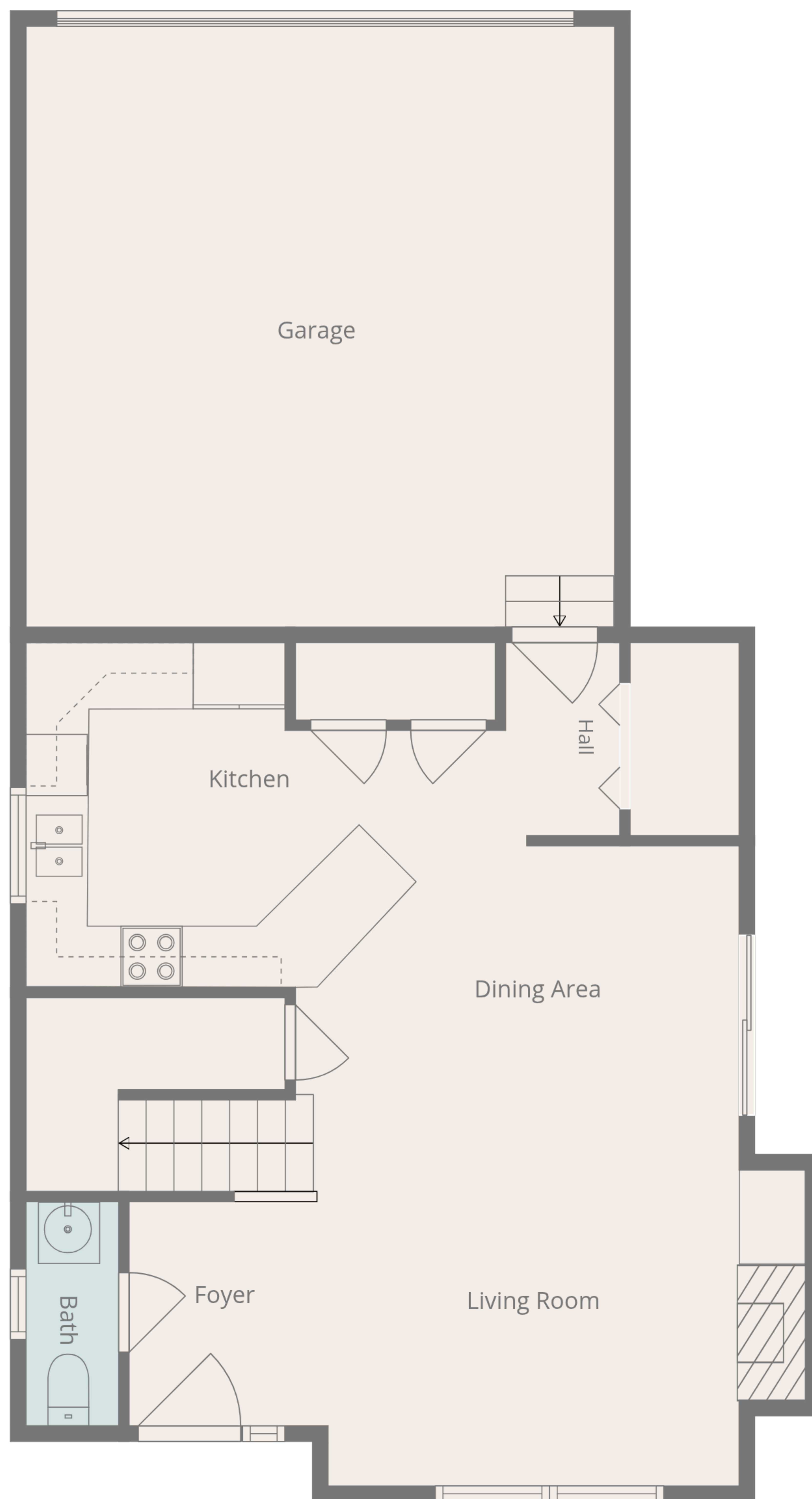
1st Floor
