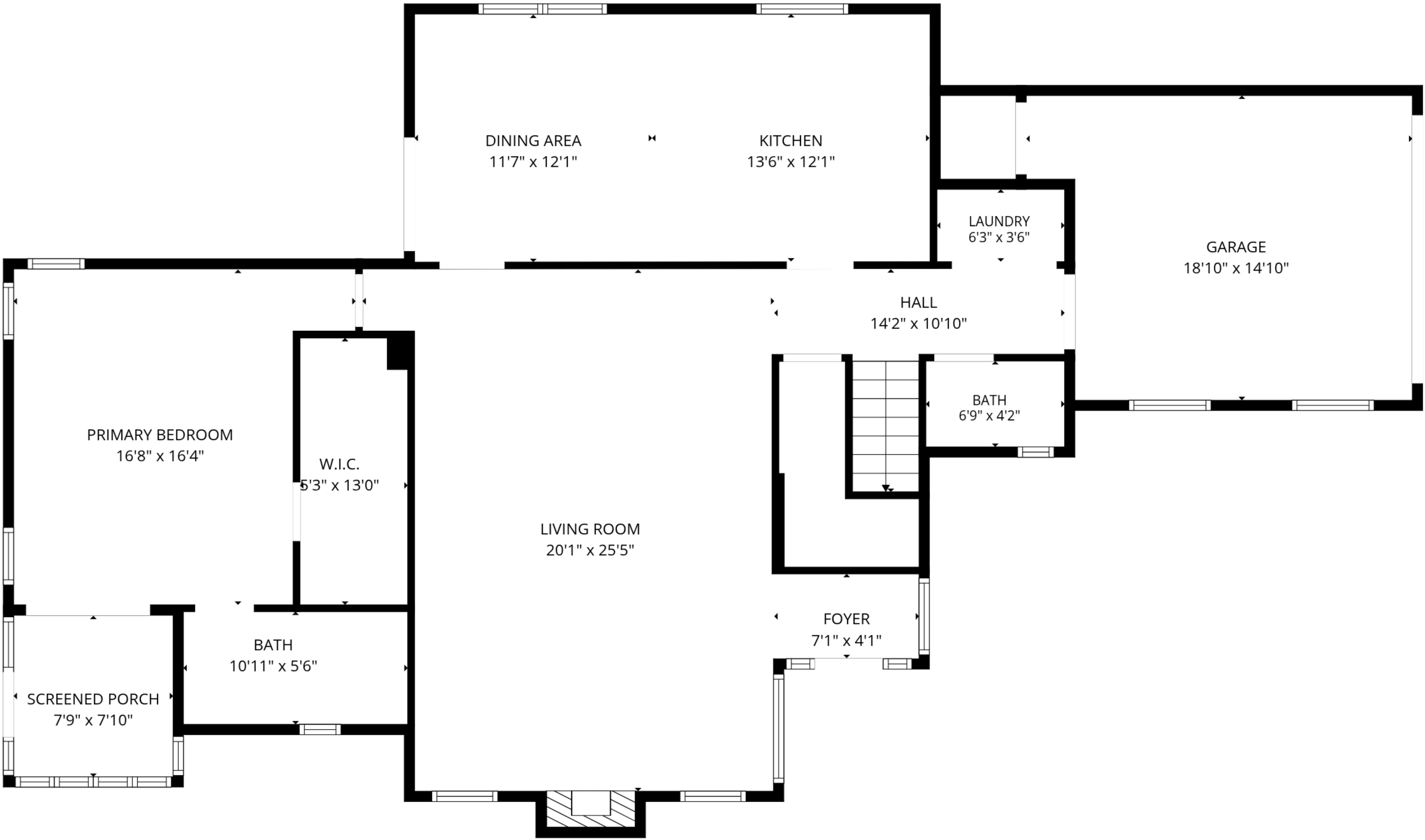
1st floor
