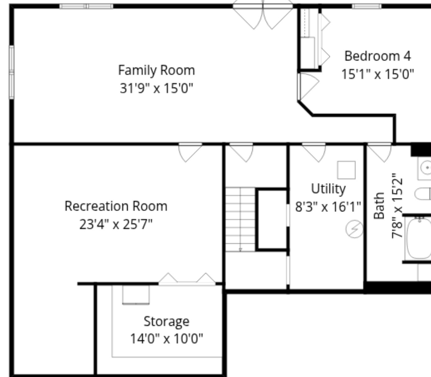
Lower Floor
