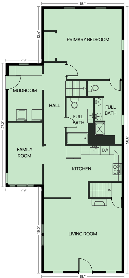
FIRST FLOOR Above grade · 8'4" ceiling · GLA 1,276 sq ft
