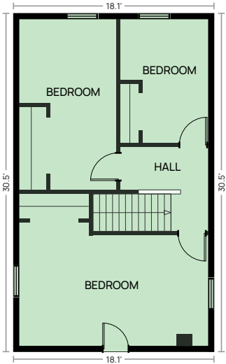
SECOND FLOOR Above grade · 8'4" ceiling GLA 552 sq ft
