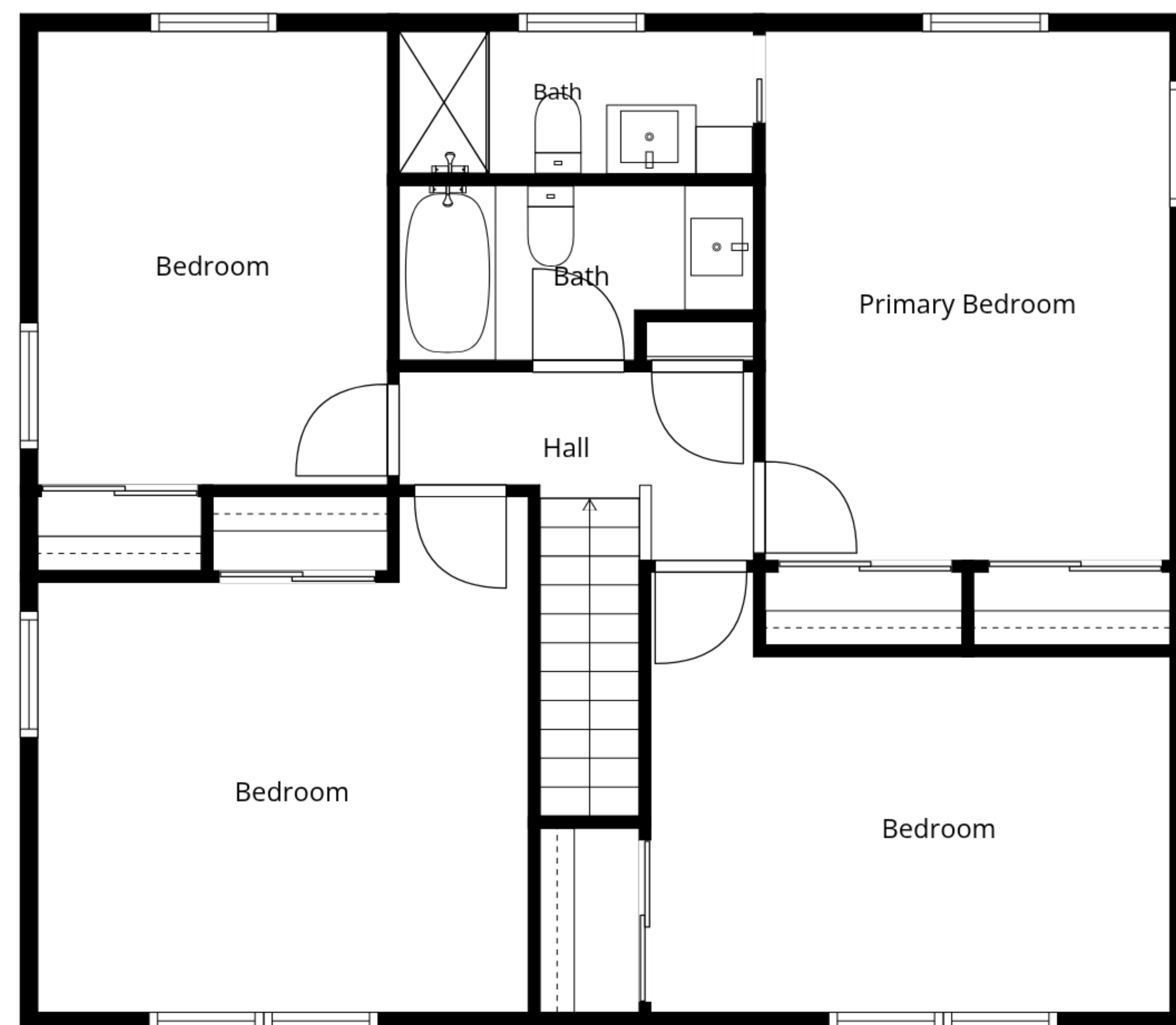
2nd Floor
