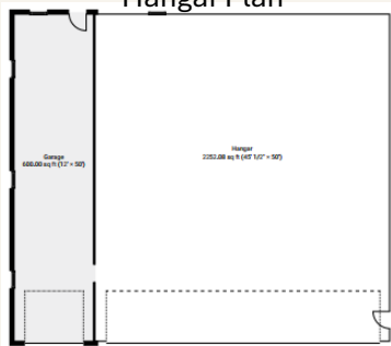
Hangar Plan
