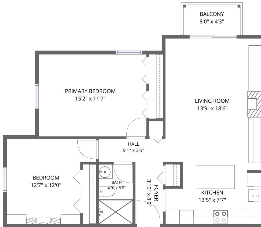
1st floor
