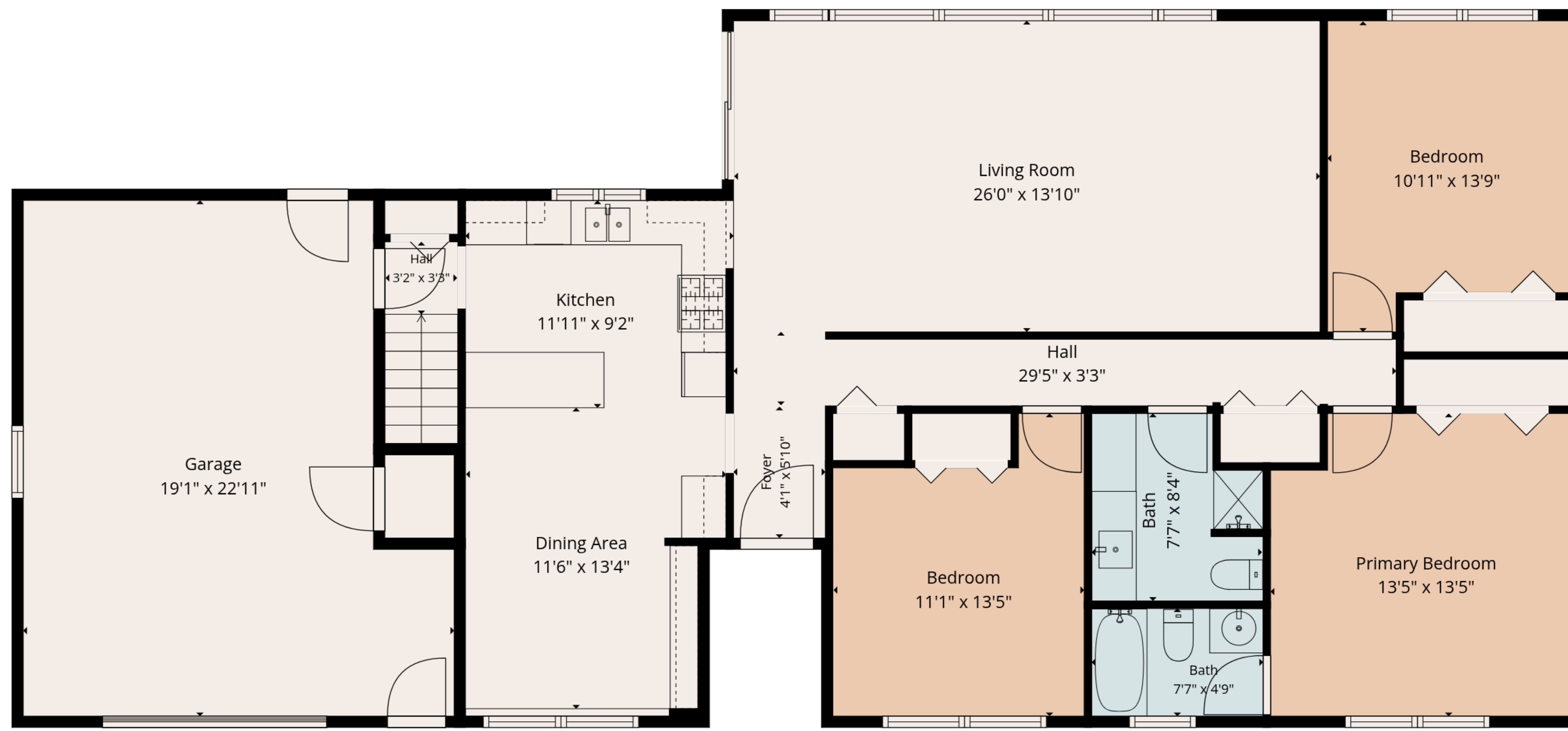
1st Floor
