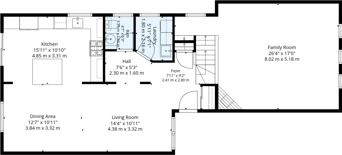
MAIN FLOOR
