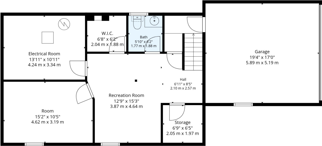
LOWER LEVEL
