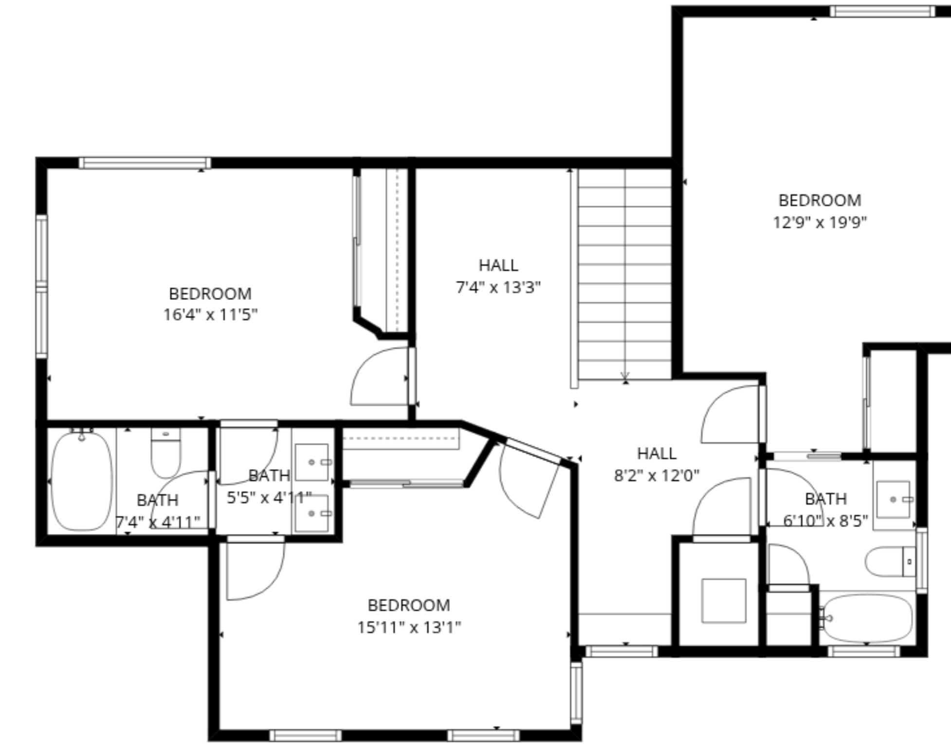
2nd floor
