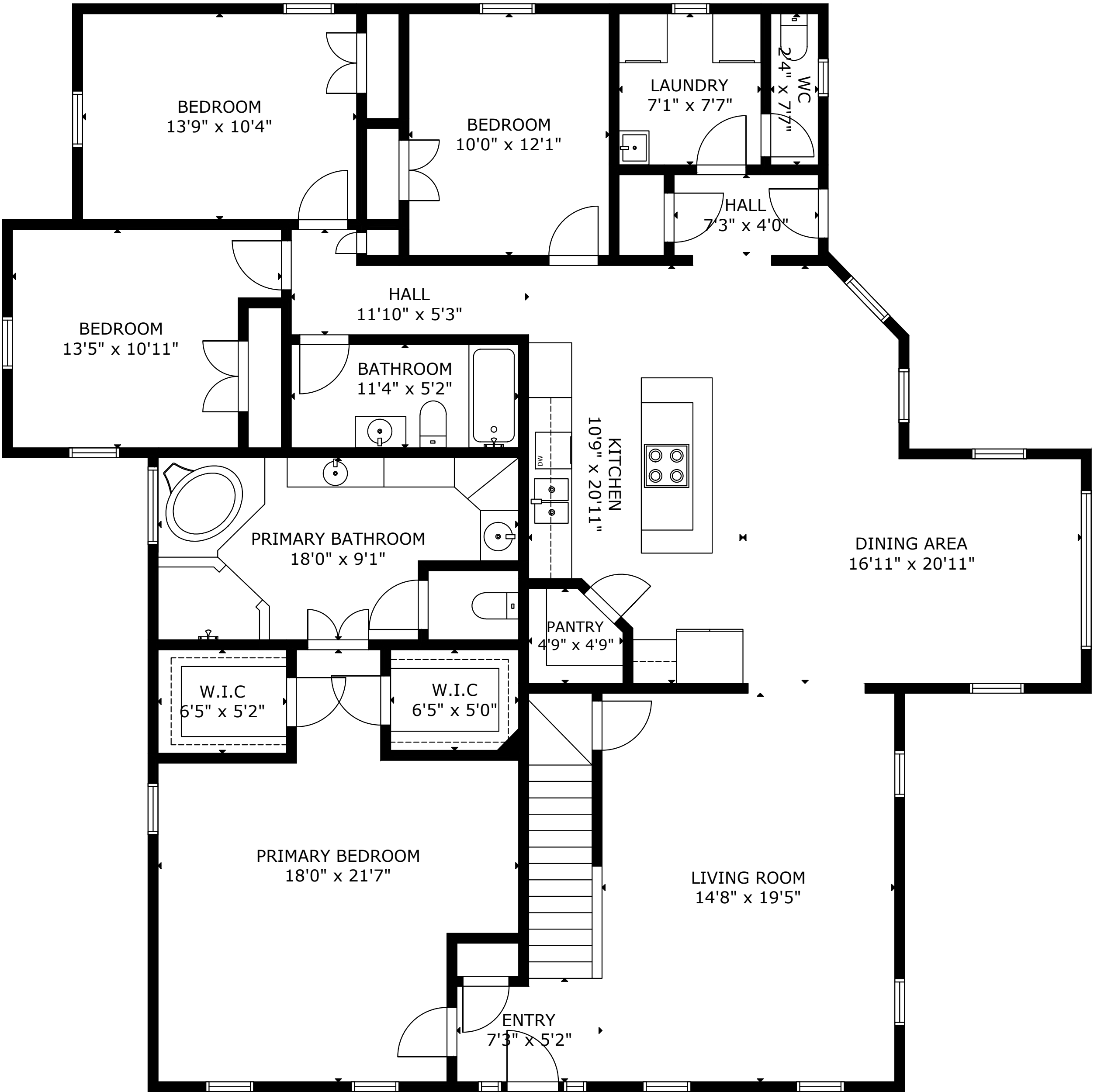
MAIN FLOOR
