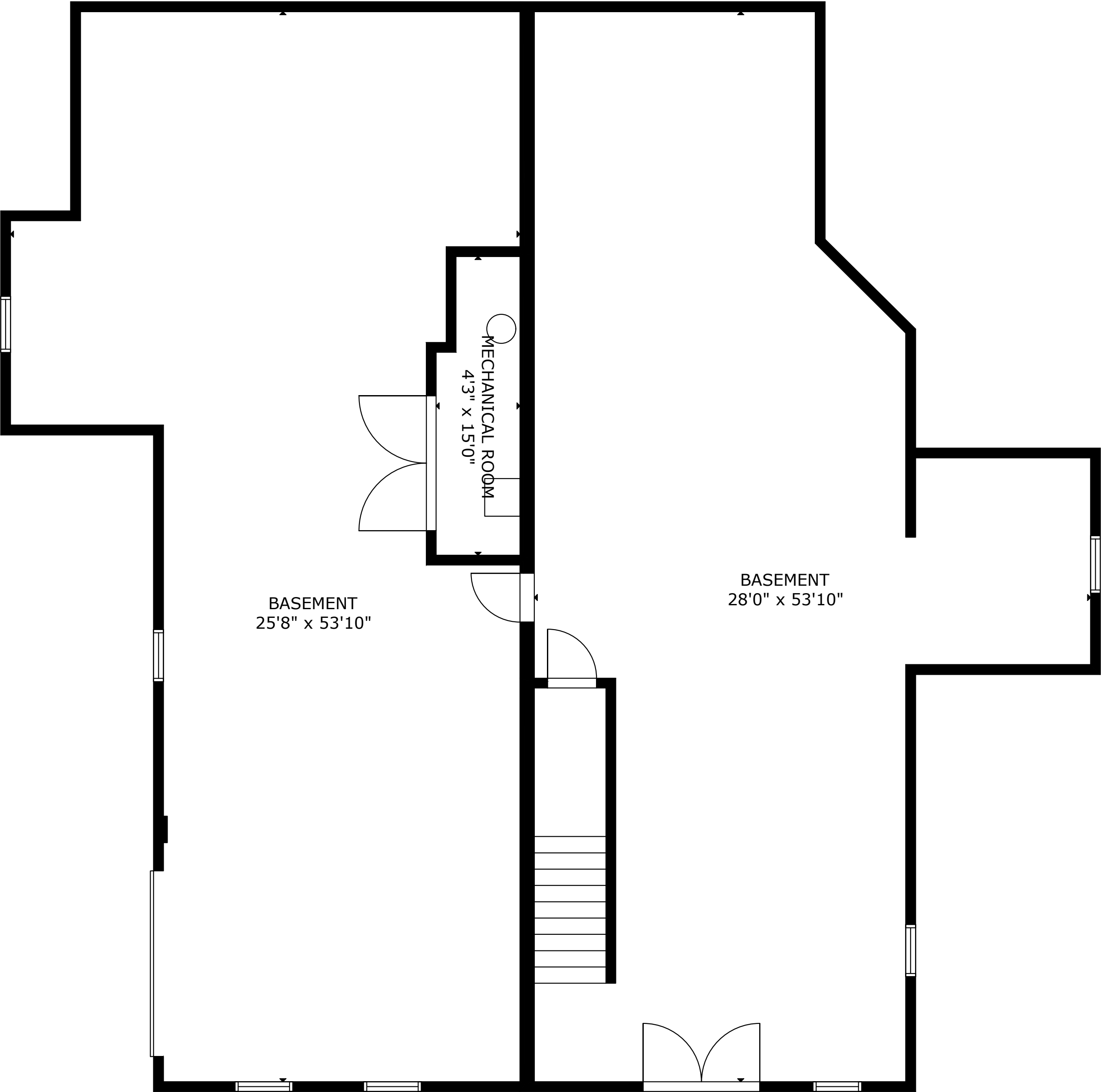
LOWER FLOOR
