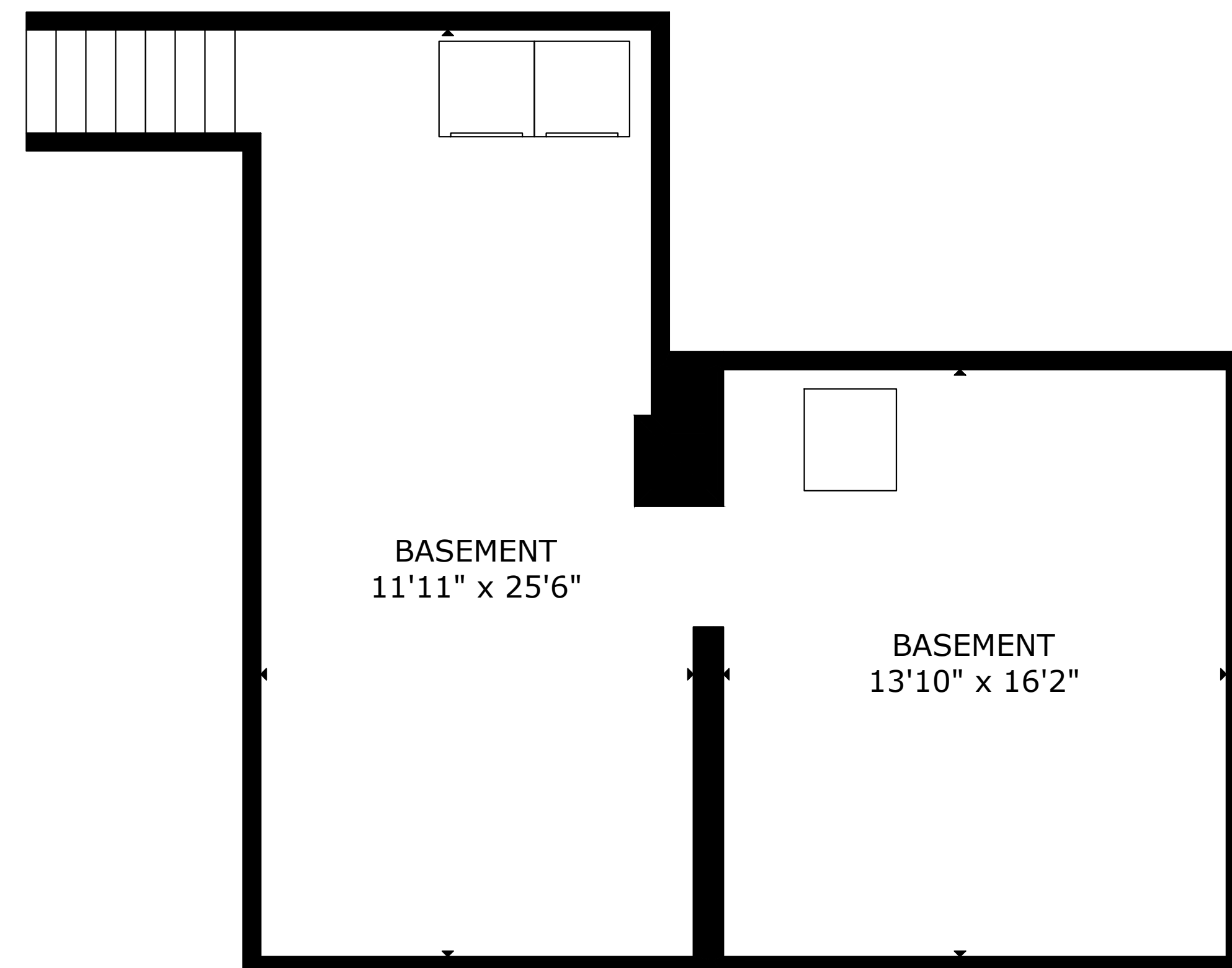
FLOOR 1
