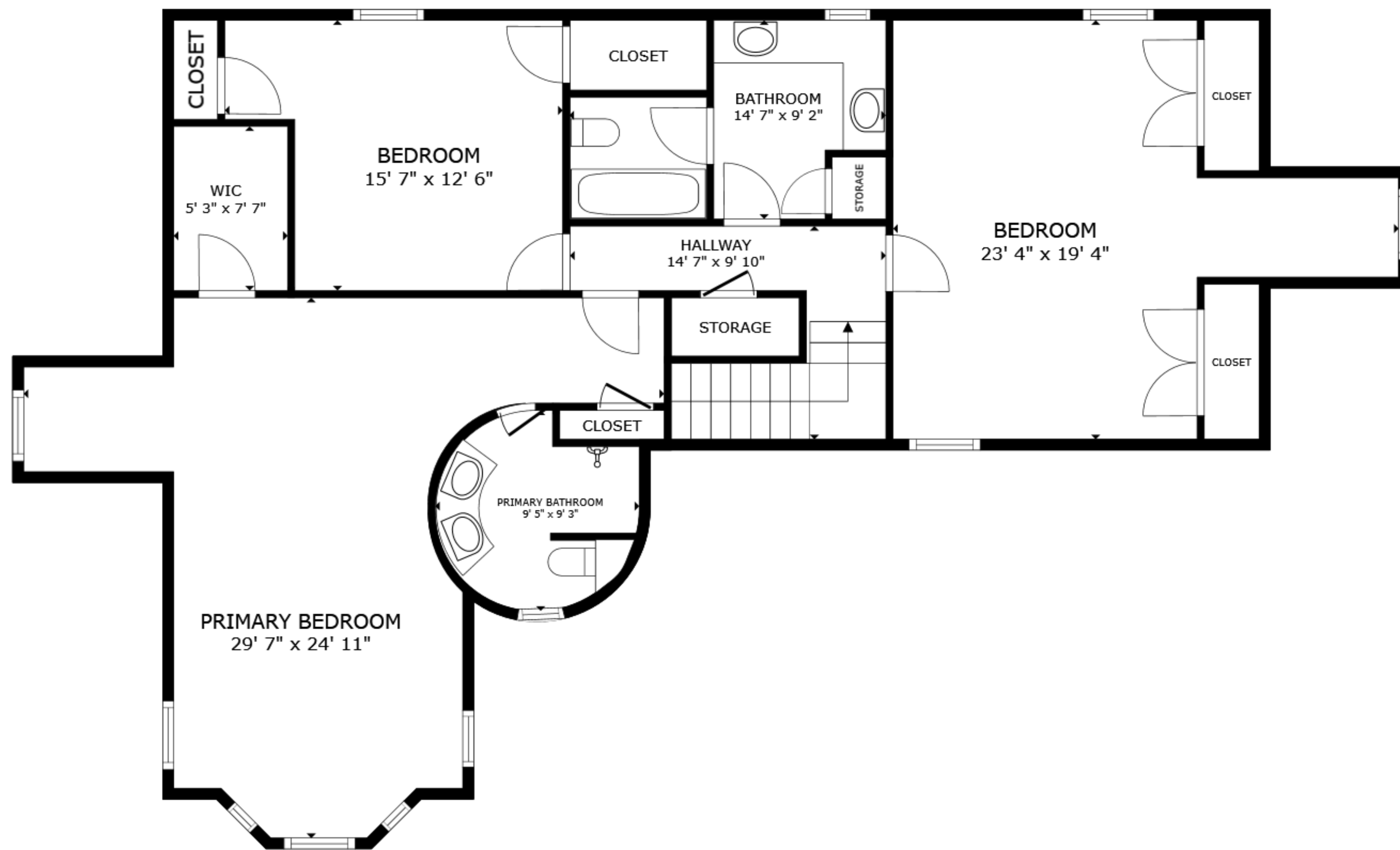
FLOOR 3
