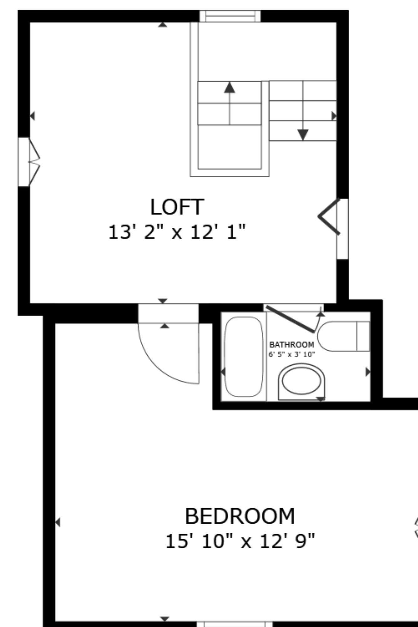
FLOOR 2
