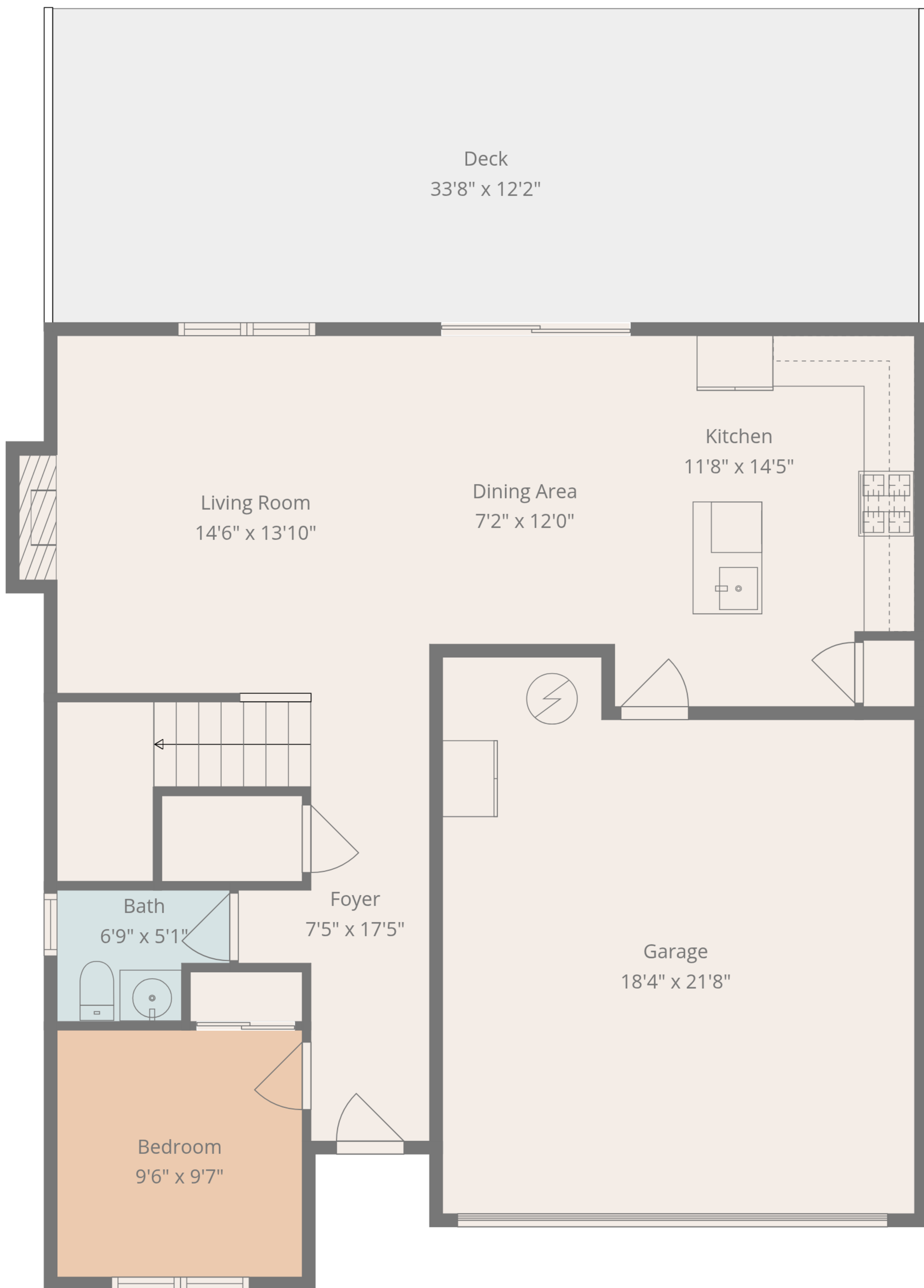
1st Floor
