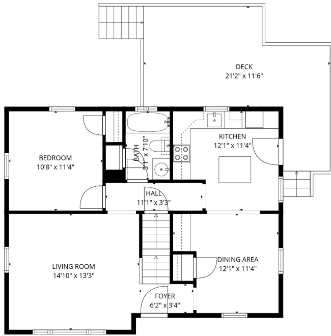
1st floor
