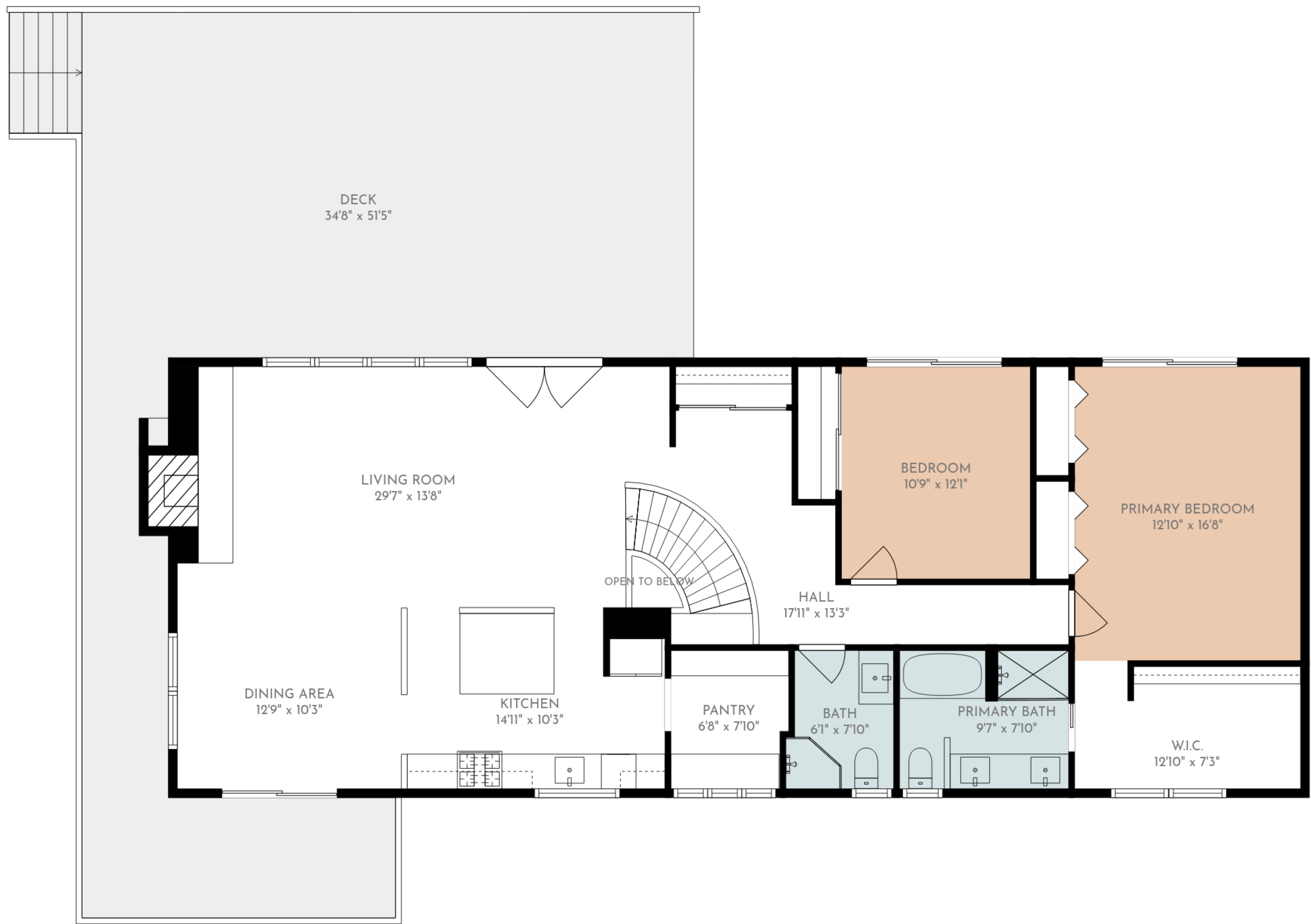
1st floor
