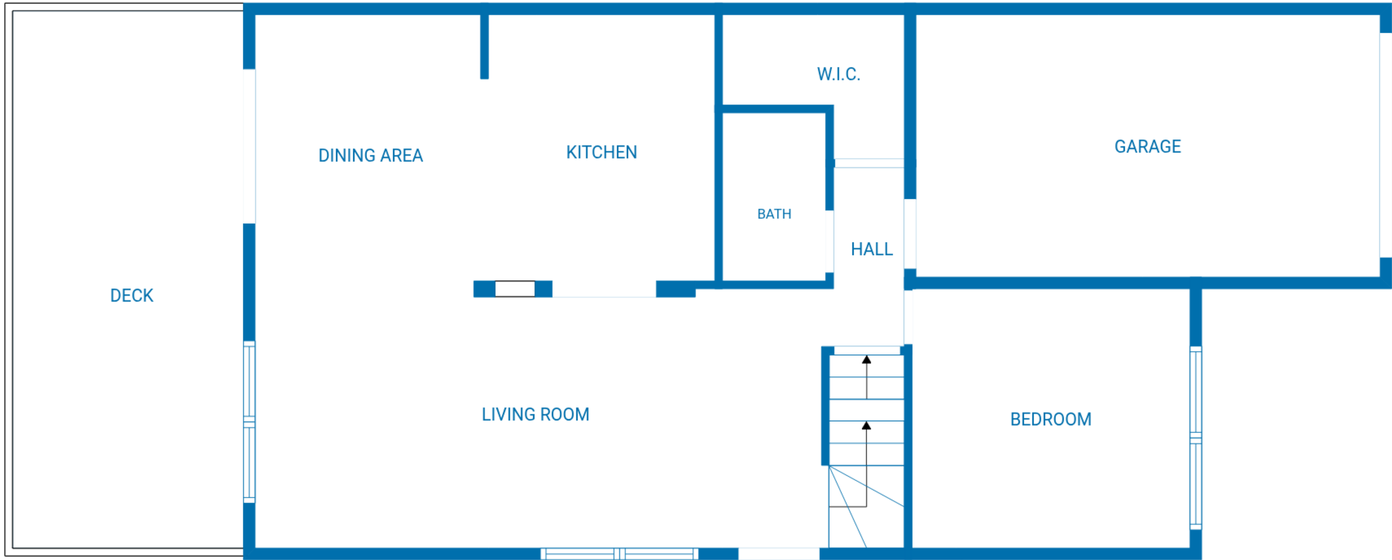
1st floor
