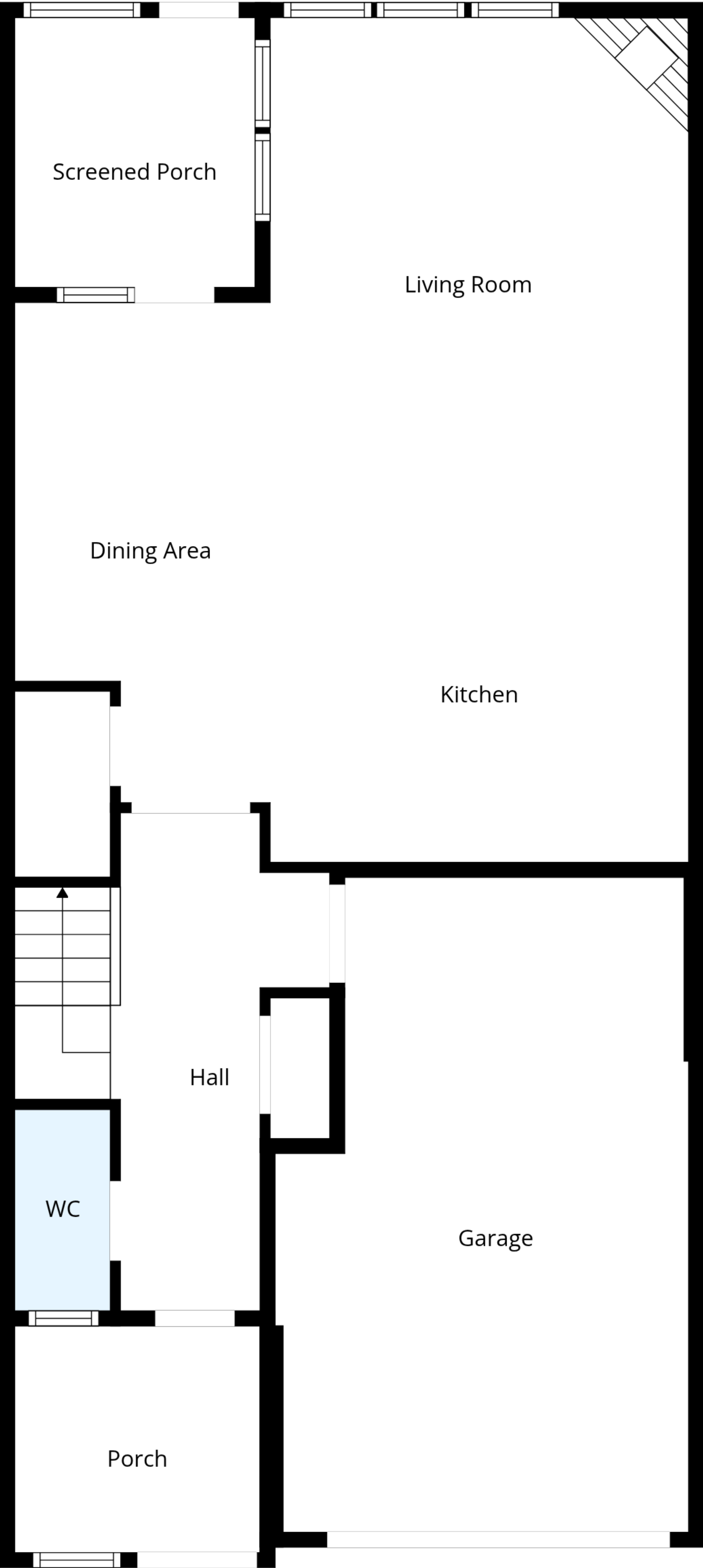
Ground Floor
