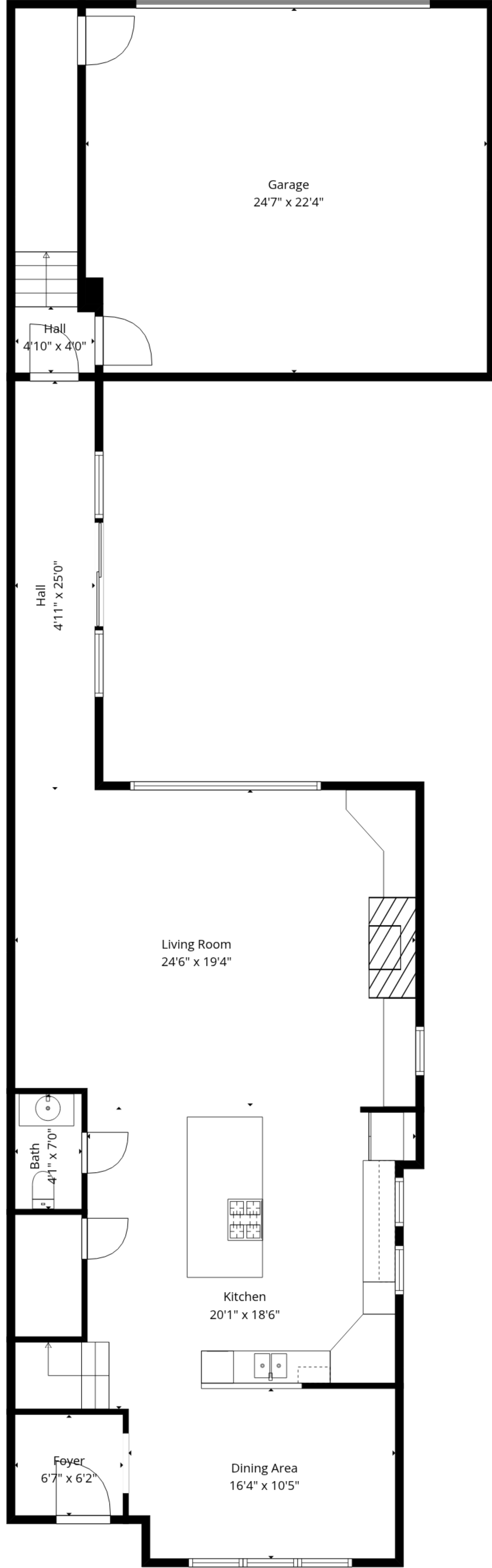
Floor 1
