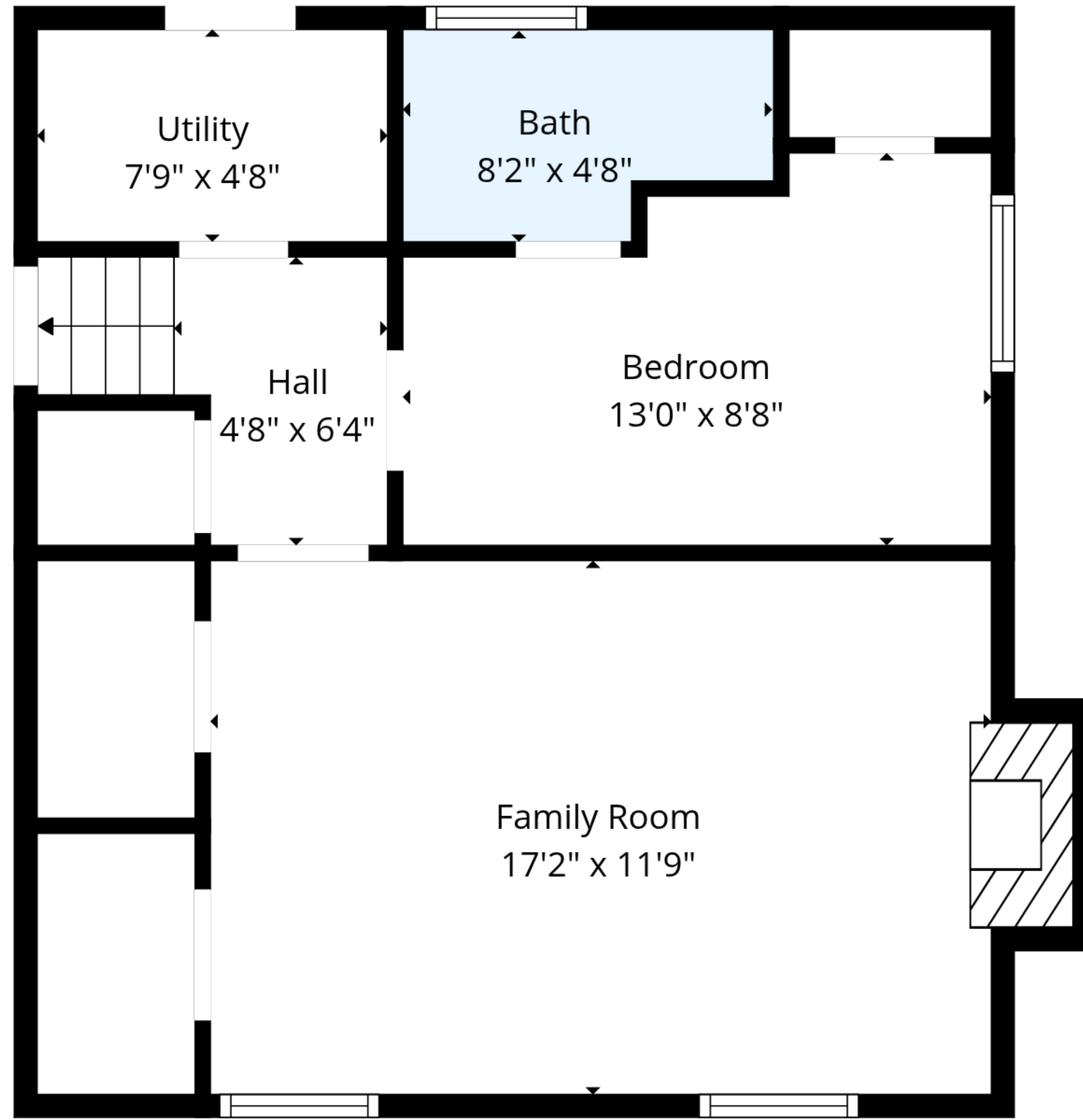
Ground Floor
