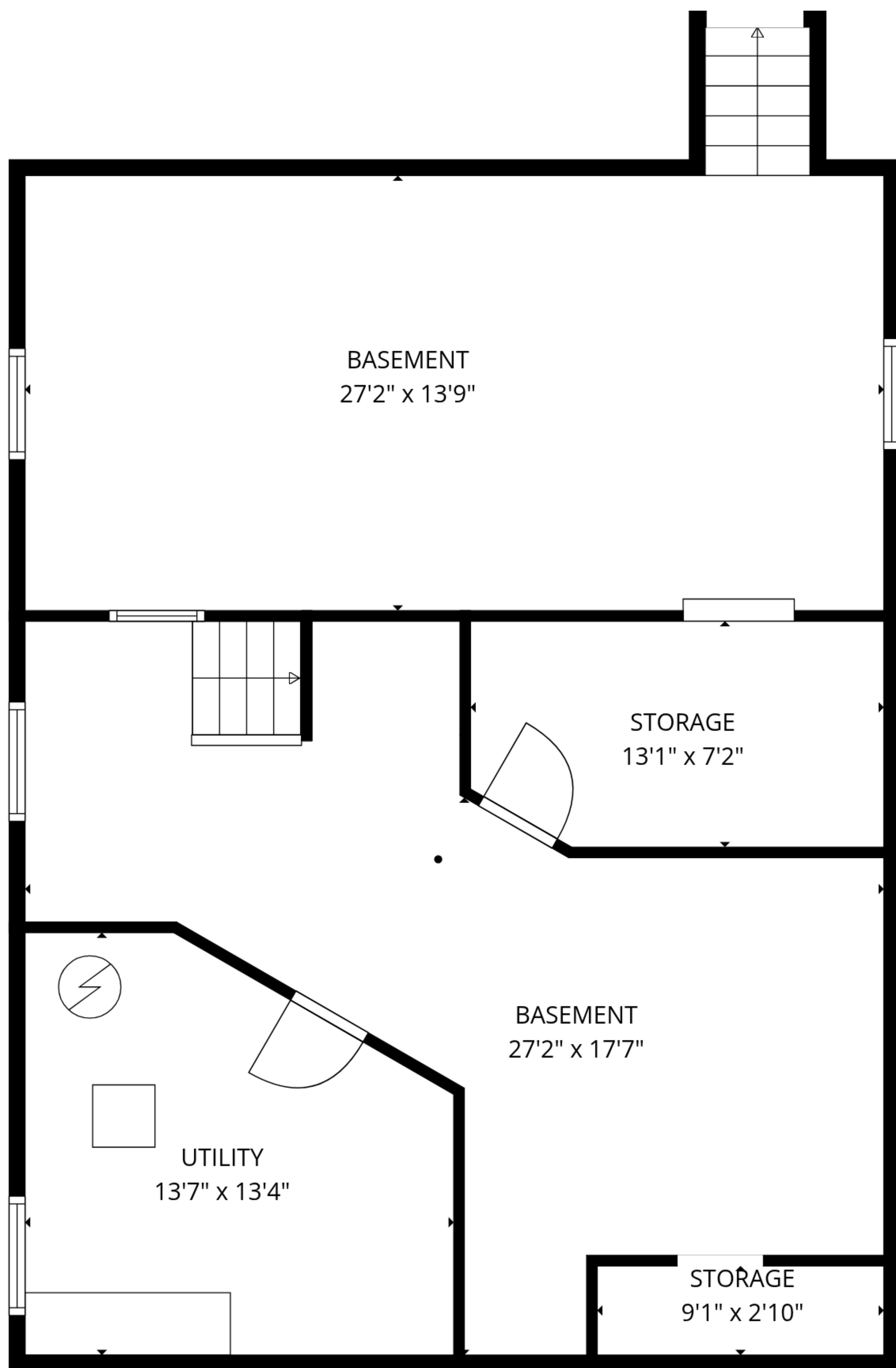
FLOOR 1
