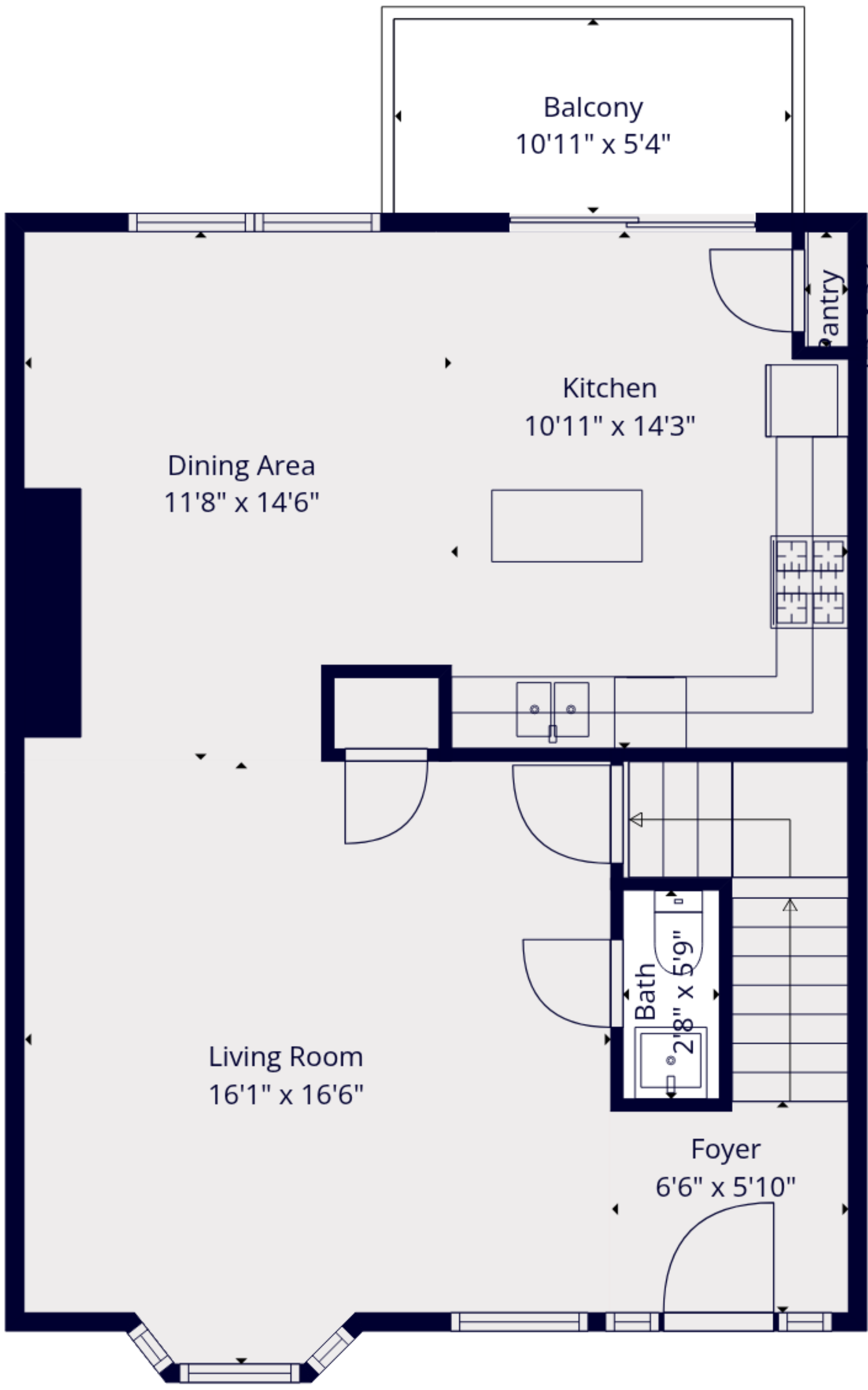
1st Floor
