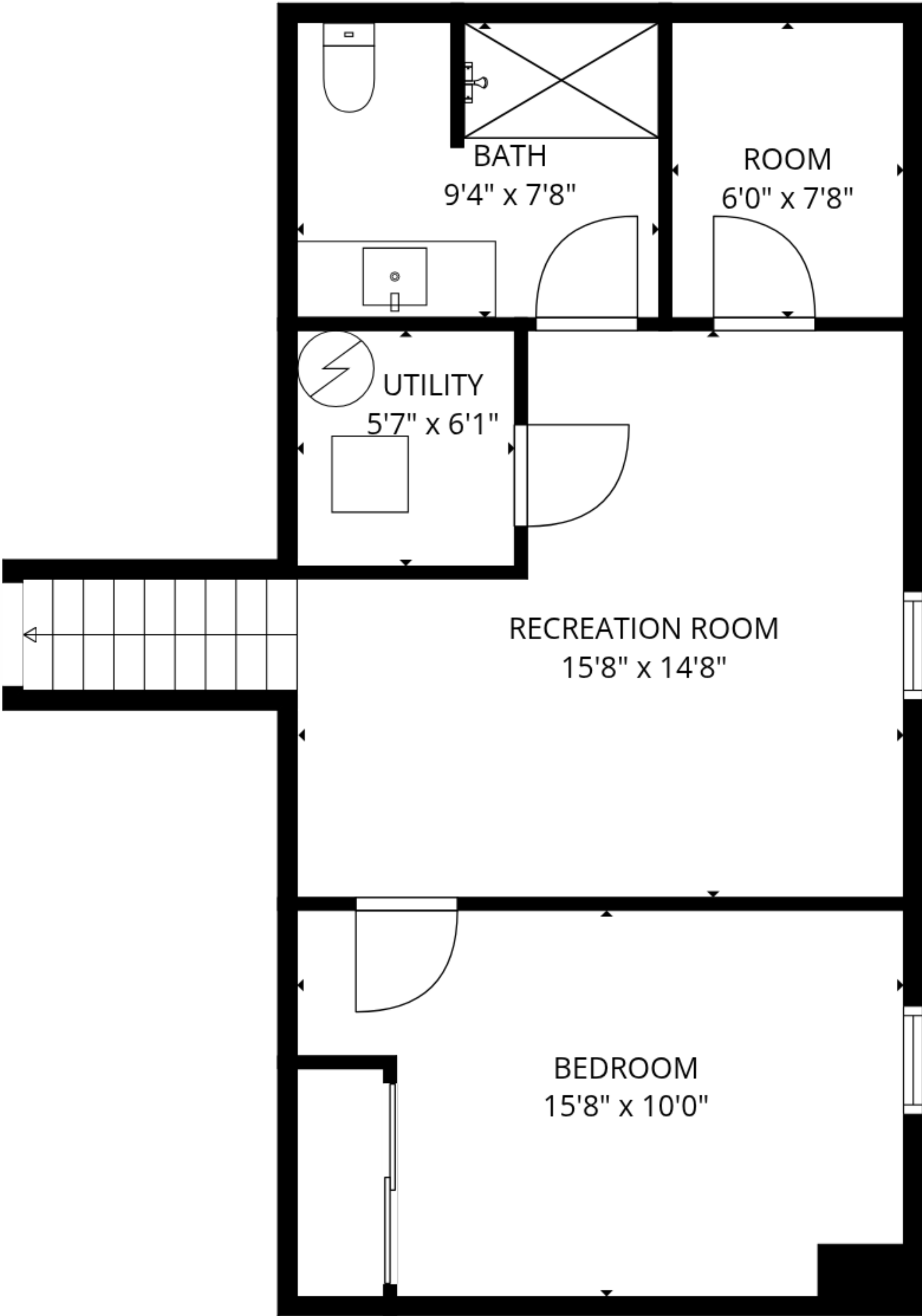
Basement 1
