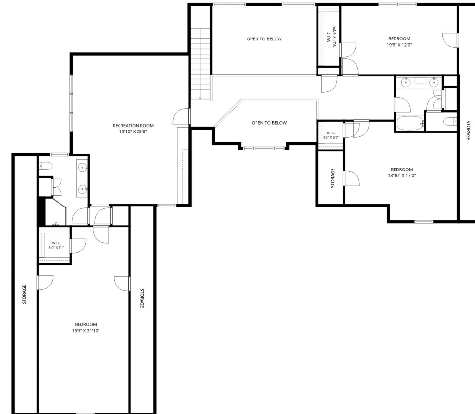
UPPER LEVEL
