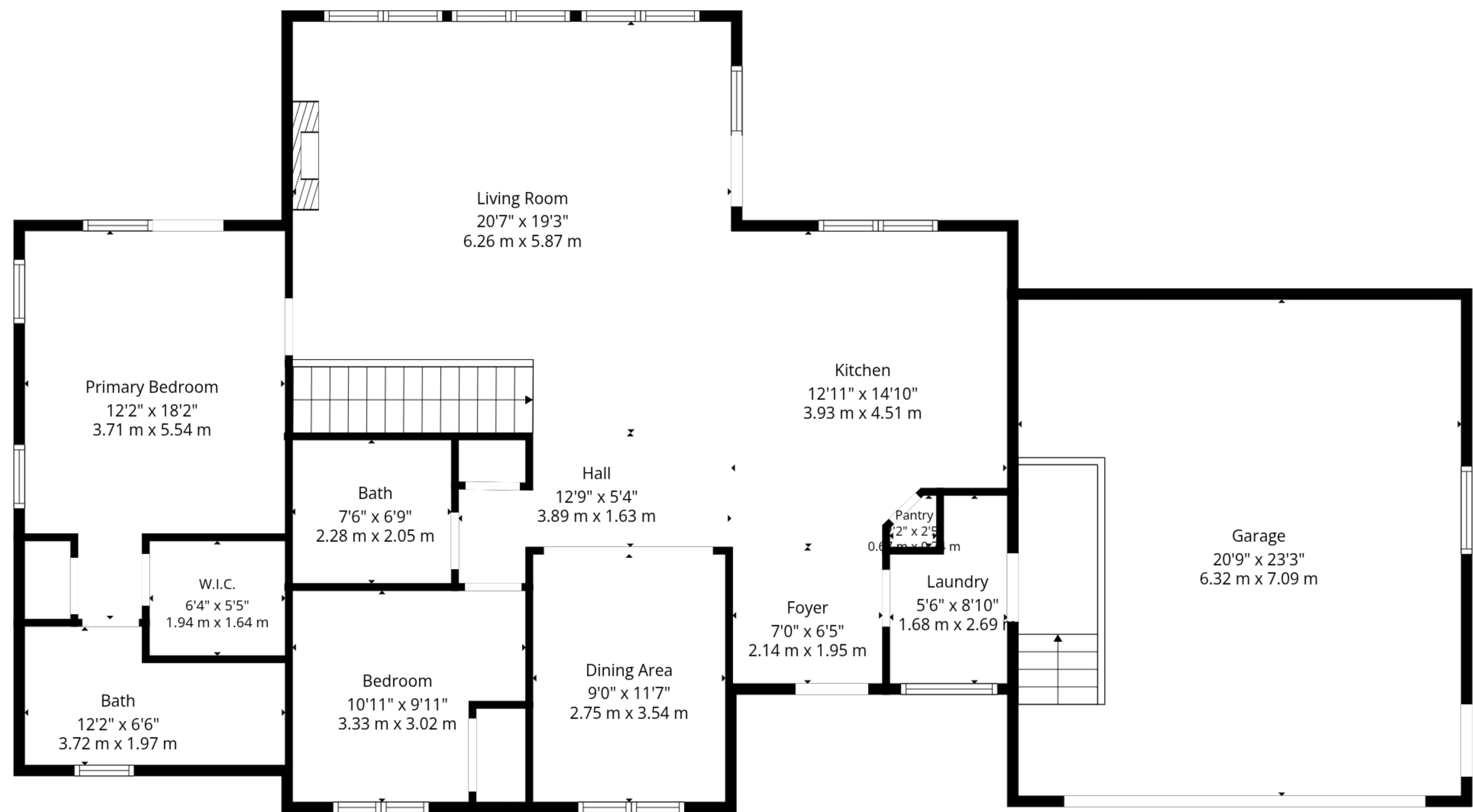
1st Floor
