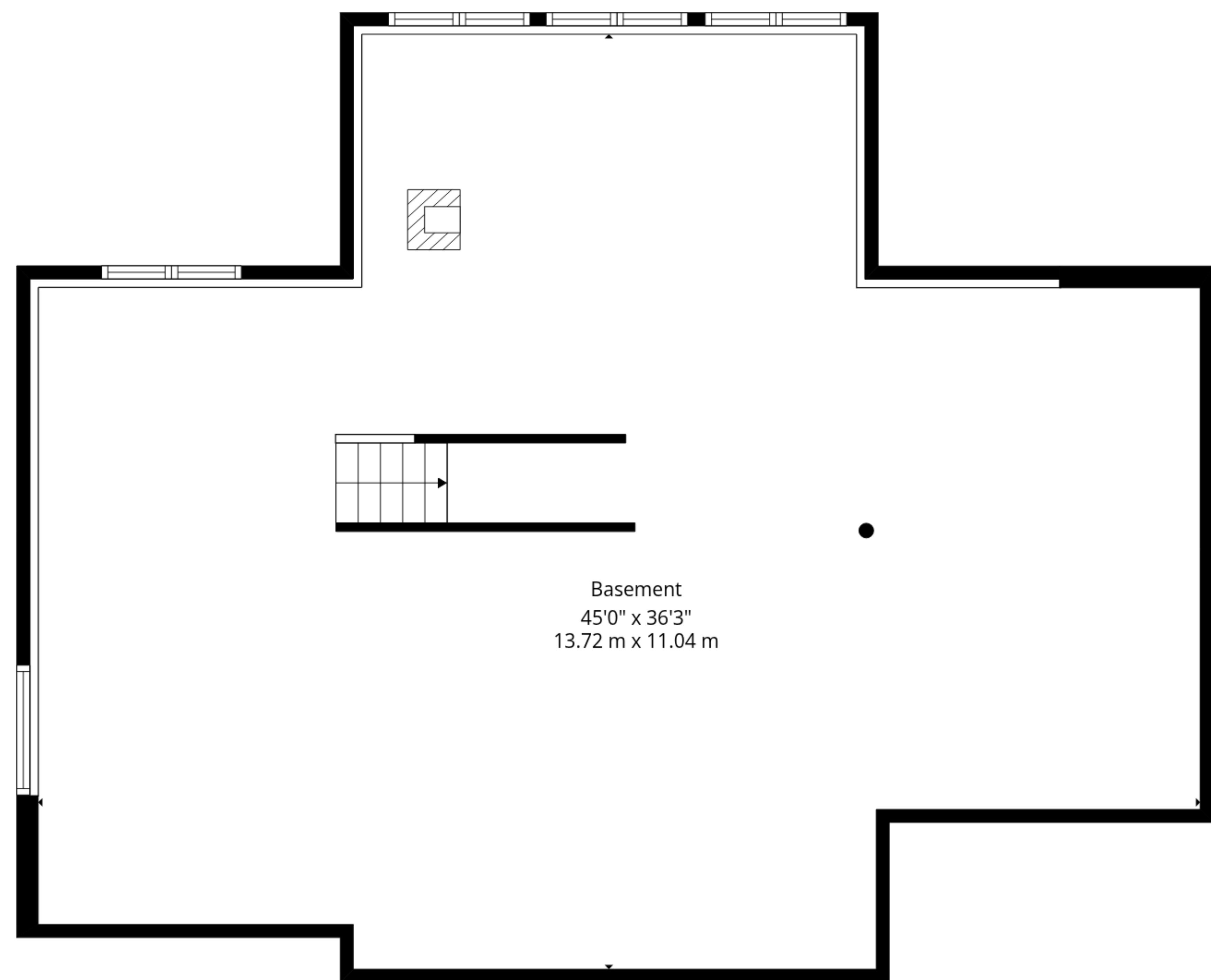
Basement
