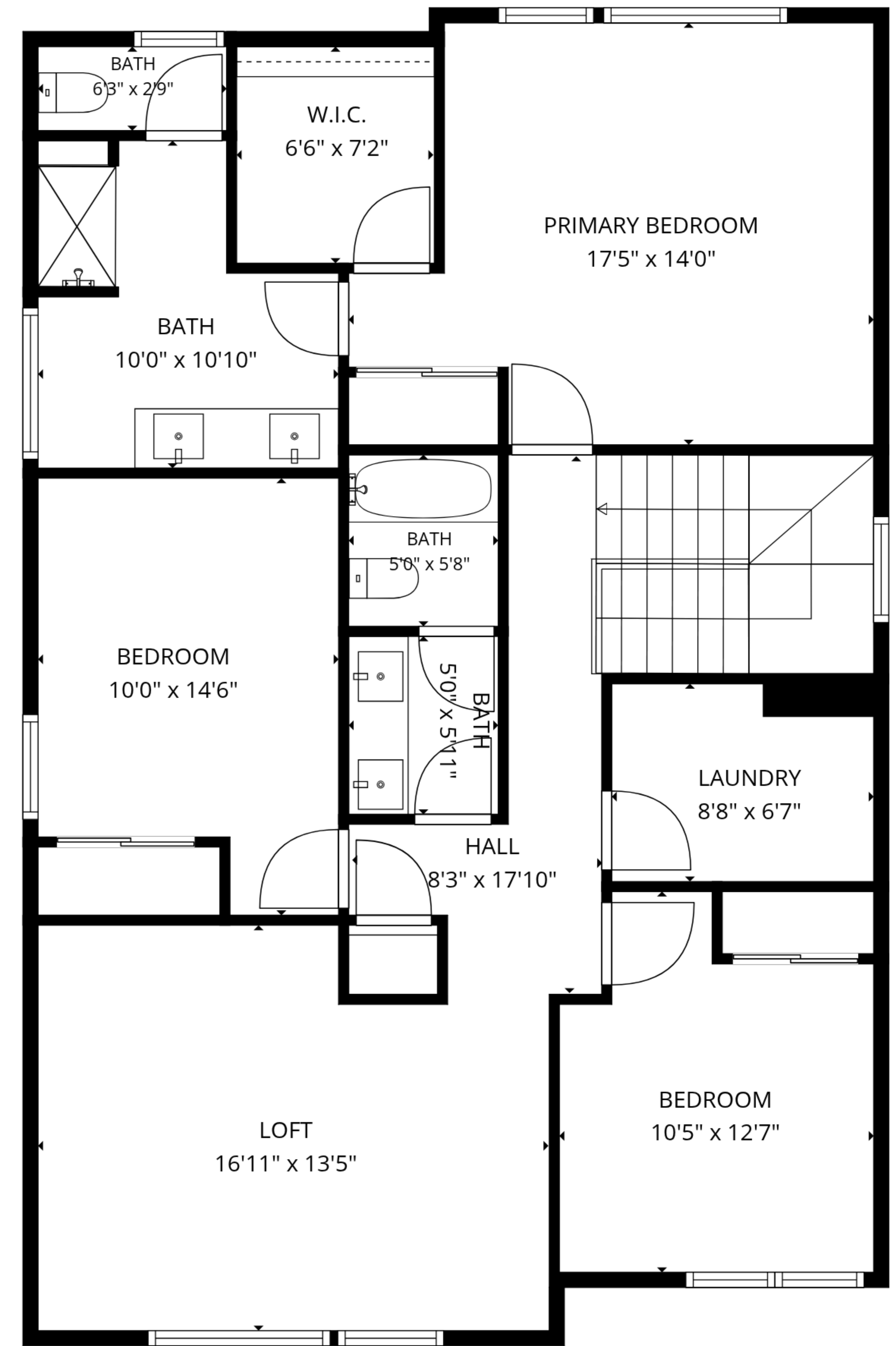
2nd floor
