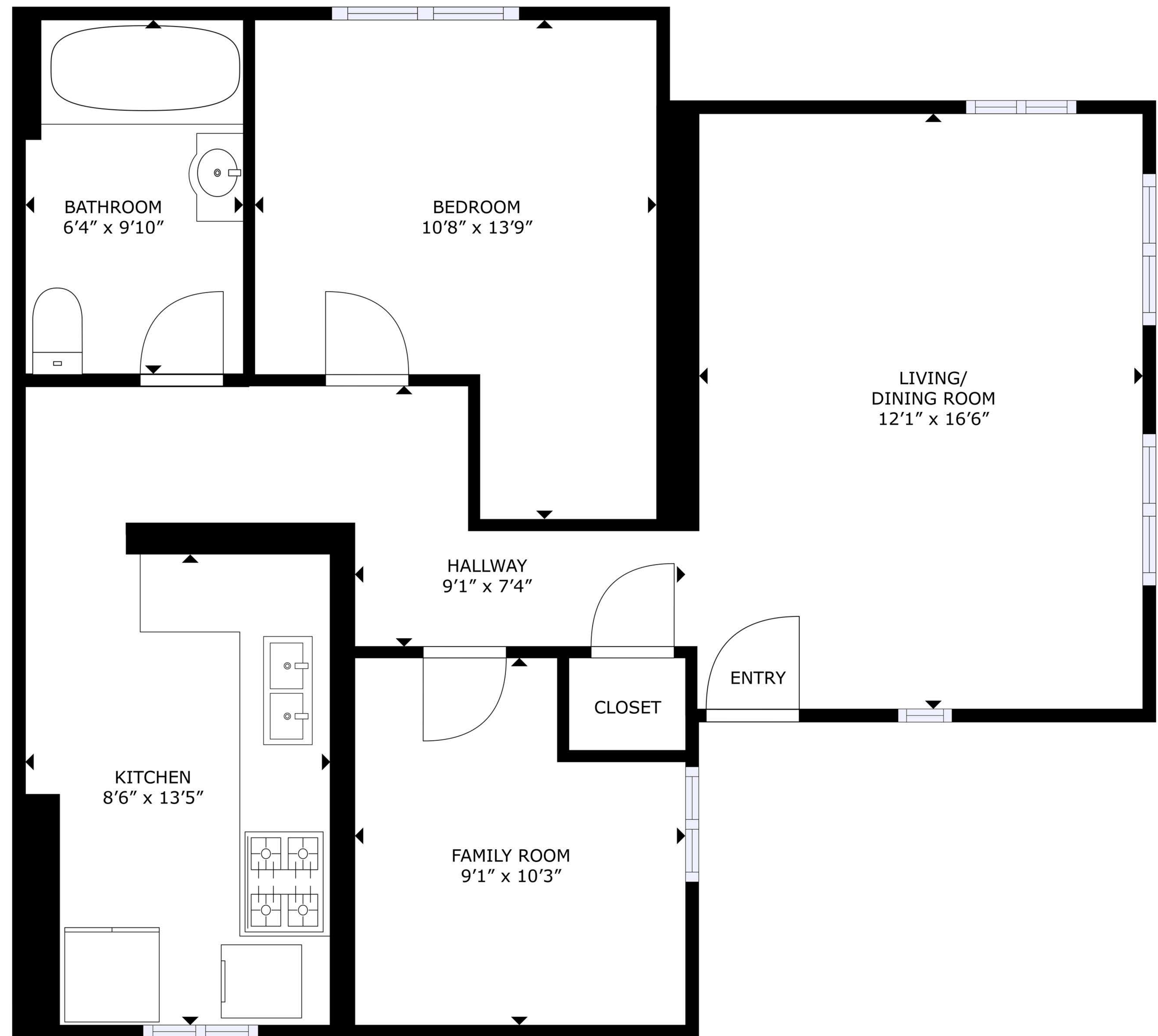
FLOOR PLAN
