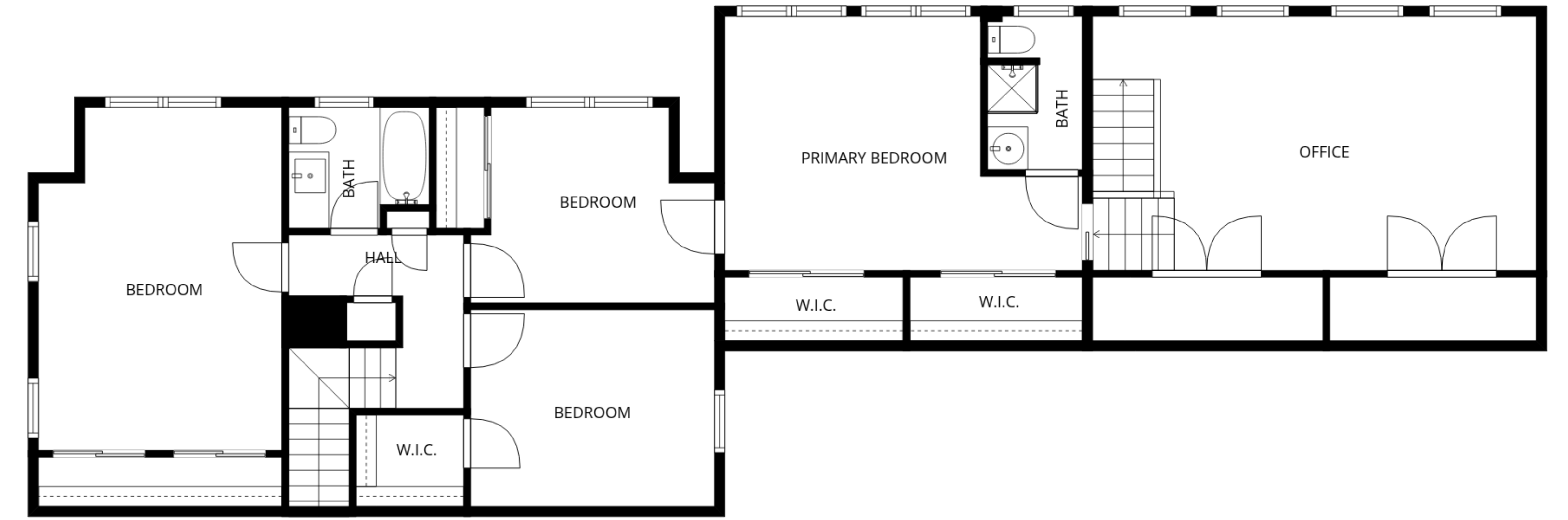
2nd floor
