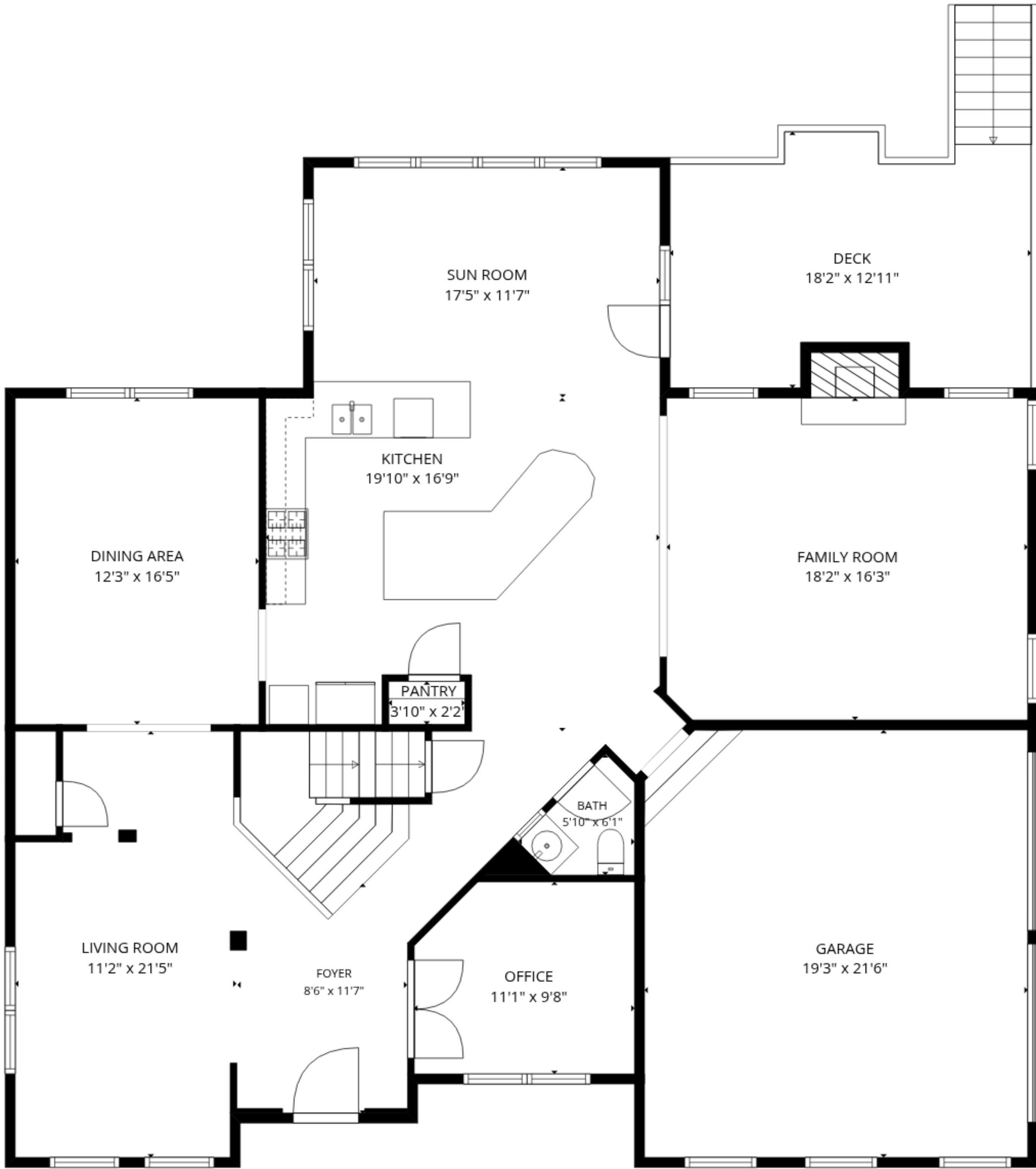
1st floor
