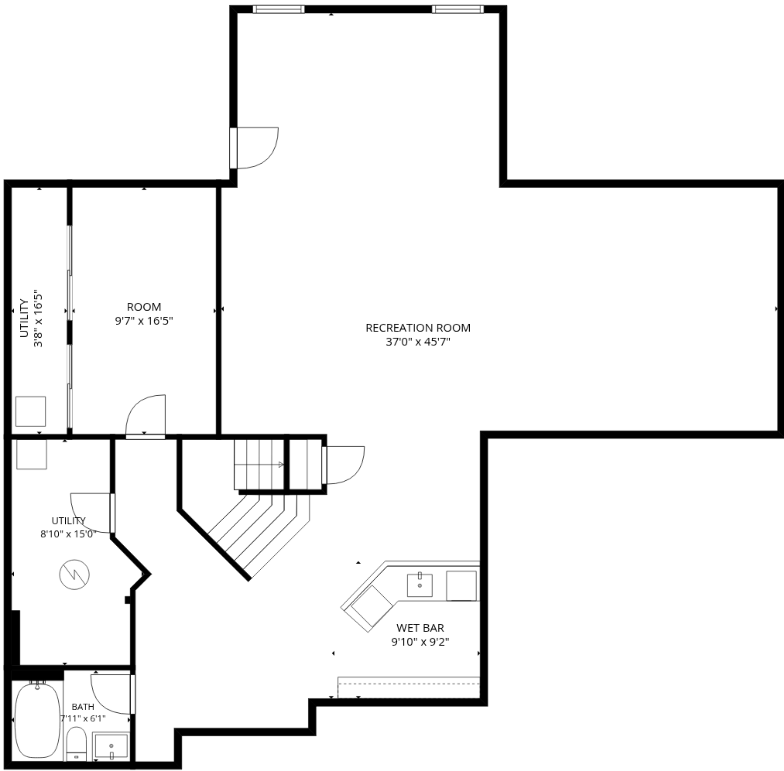
Basement
