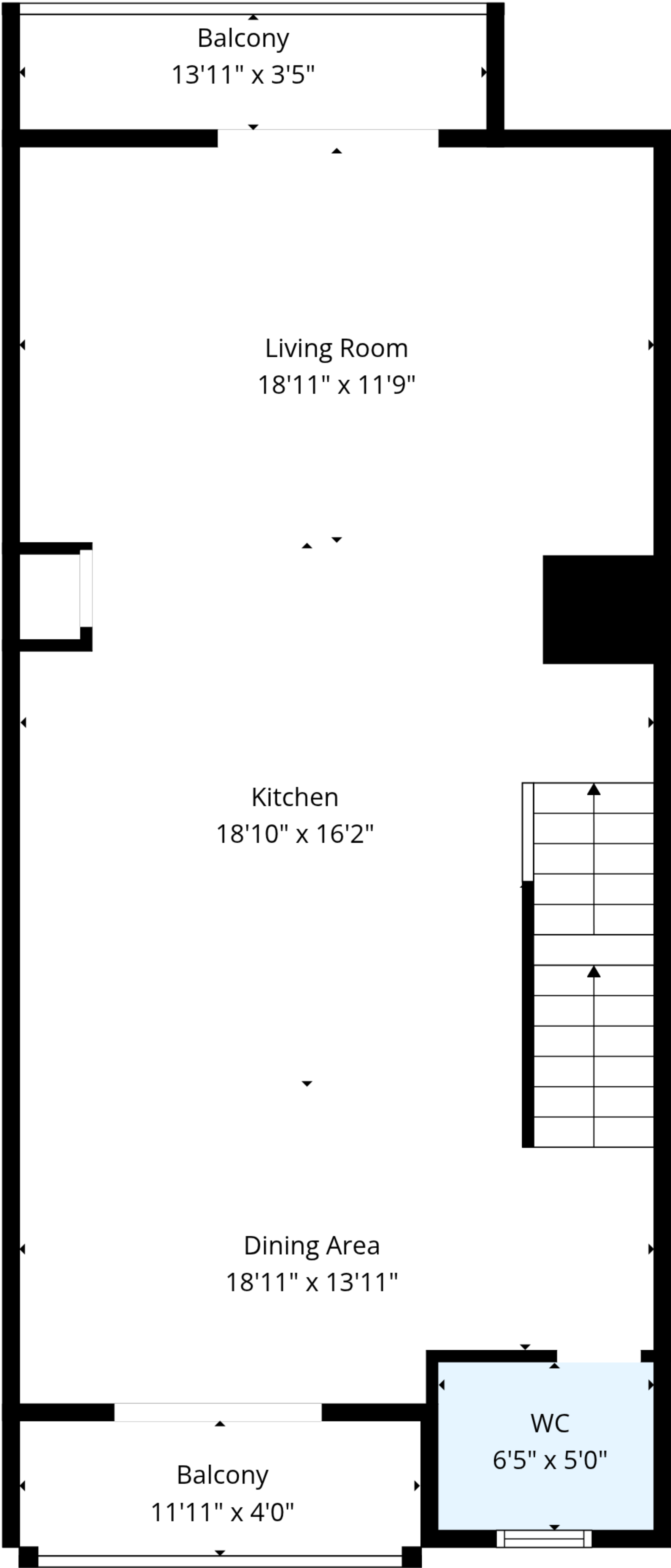
1st Floor
