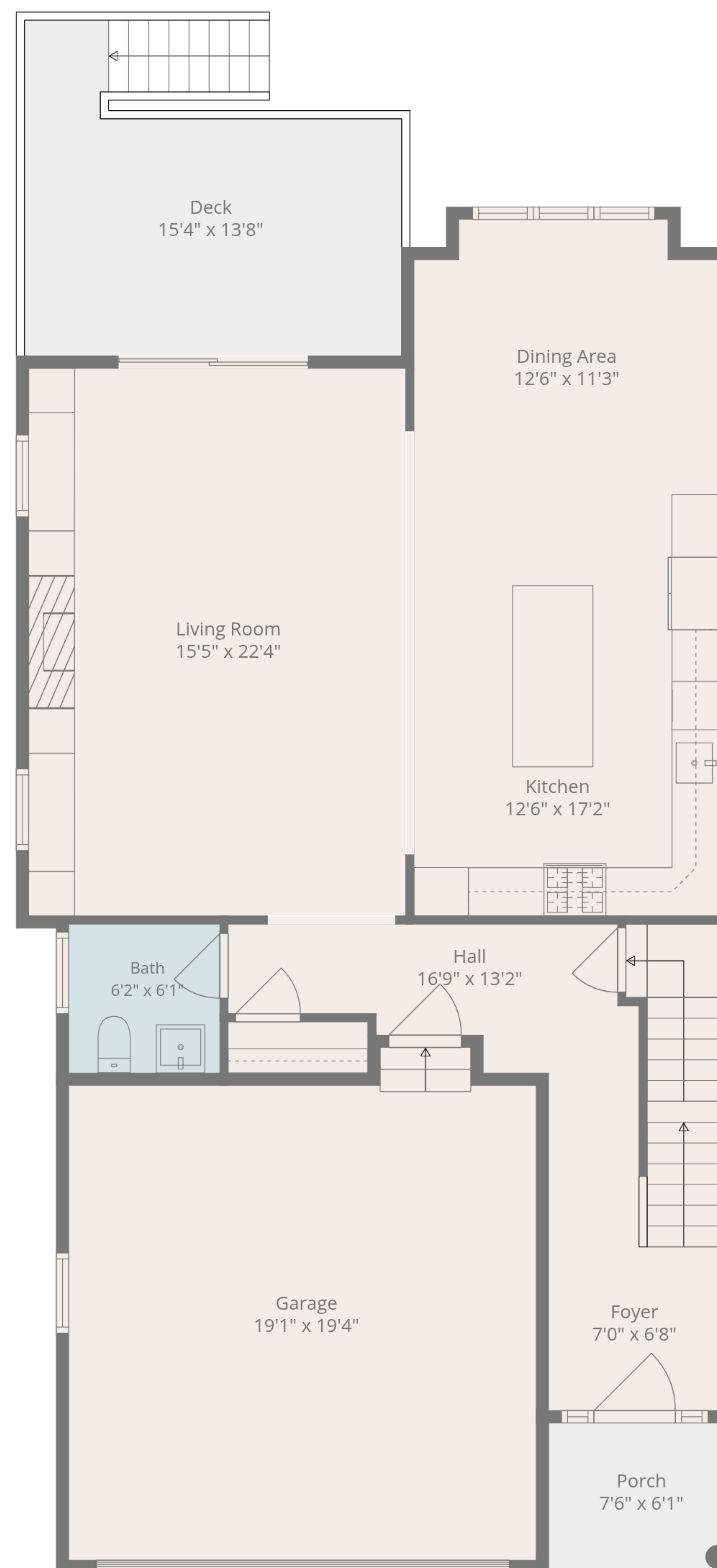
1st Floor
