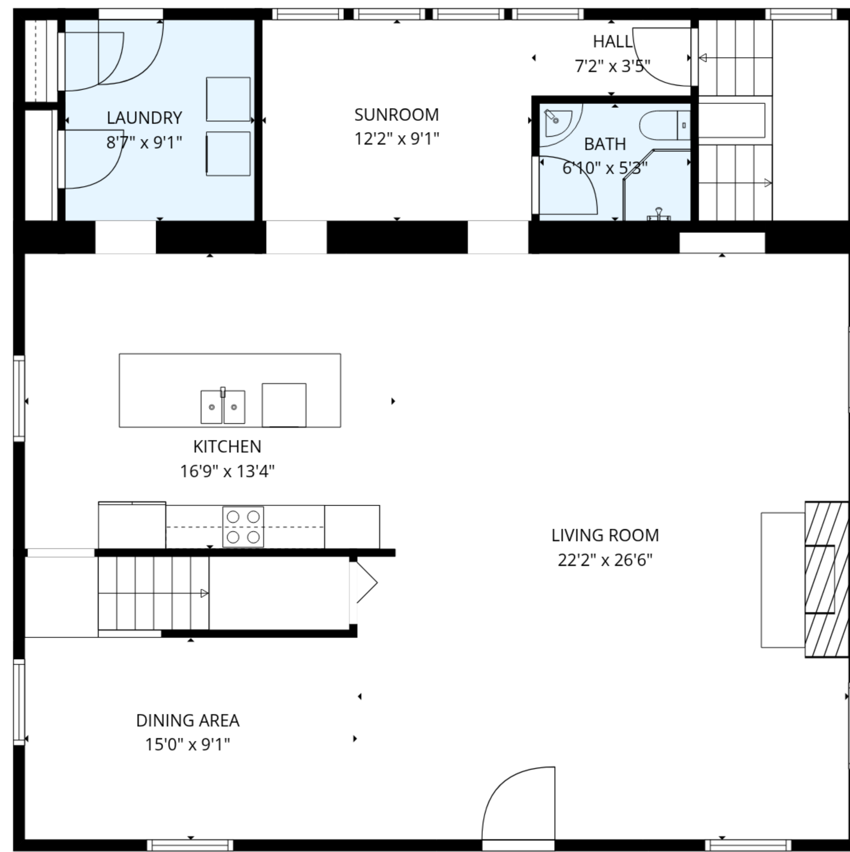
1st floor
