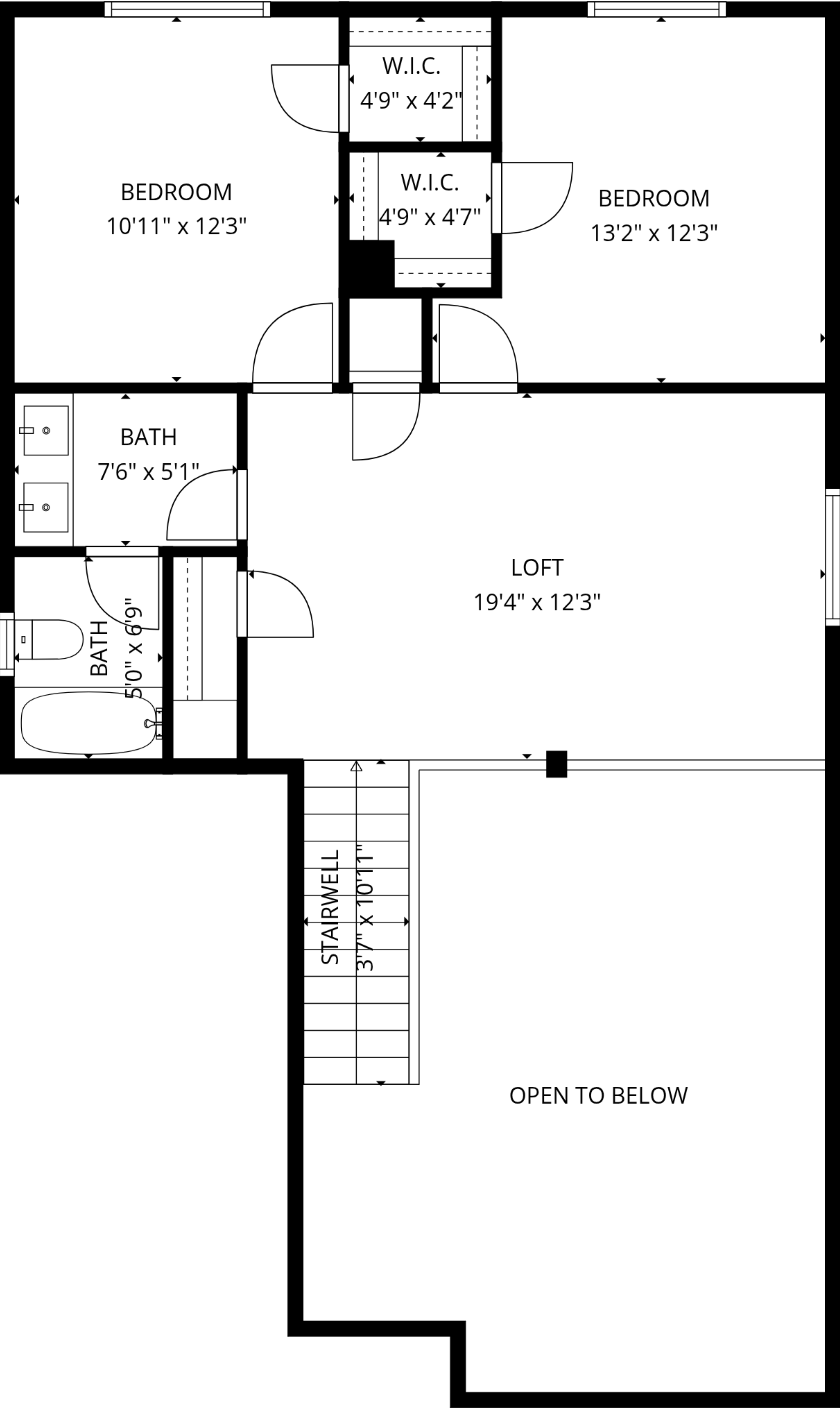
FLOOR 2
