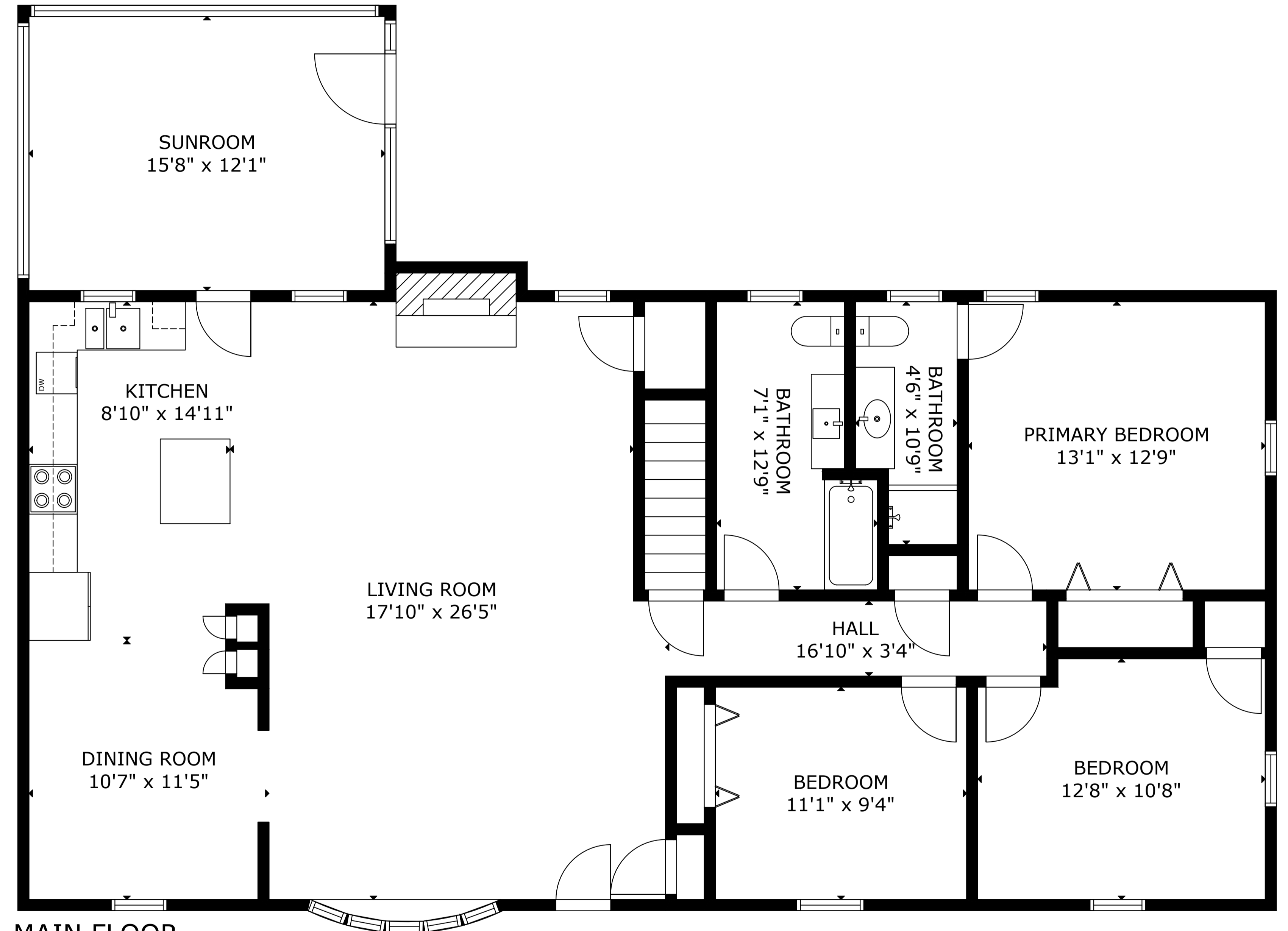
MAIN FLOOR
