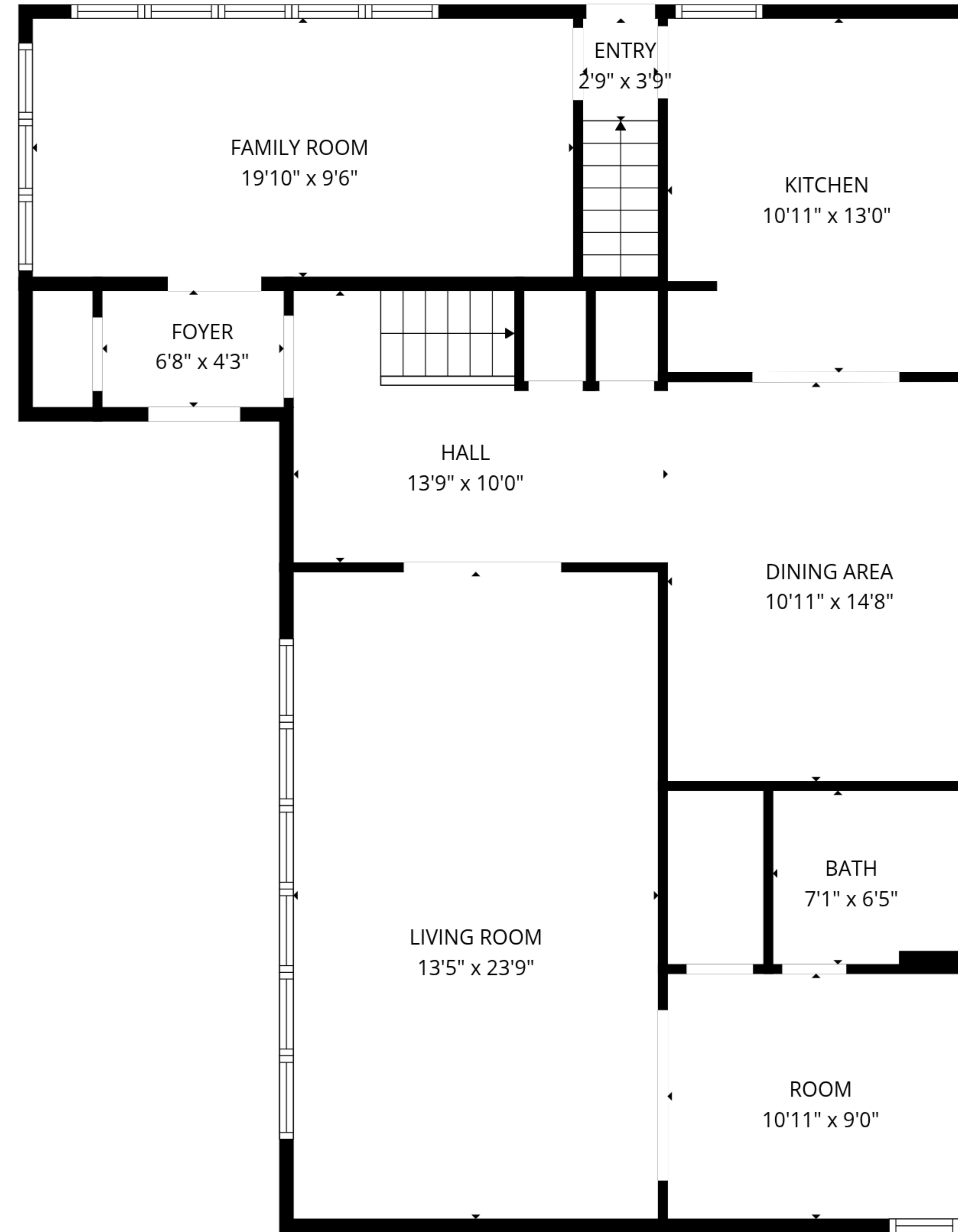
1st floor
