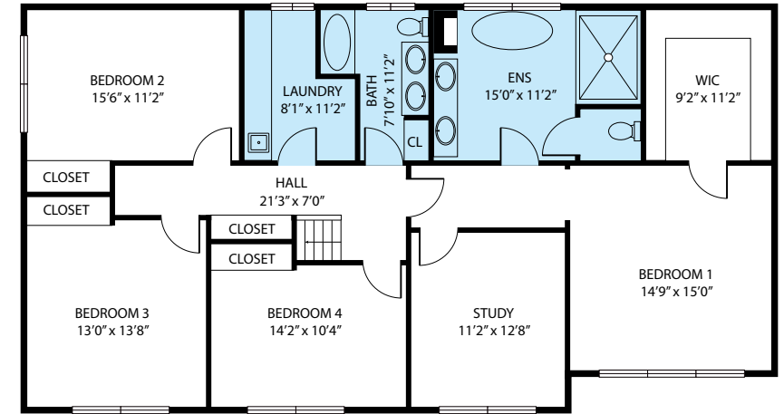
SECOND FLOOR
