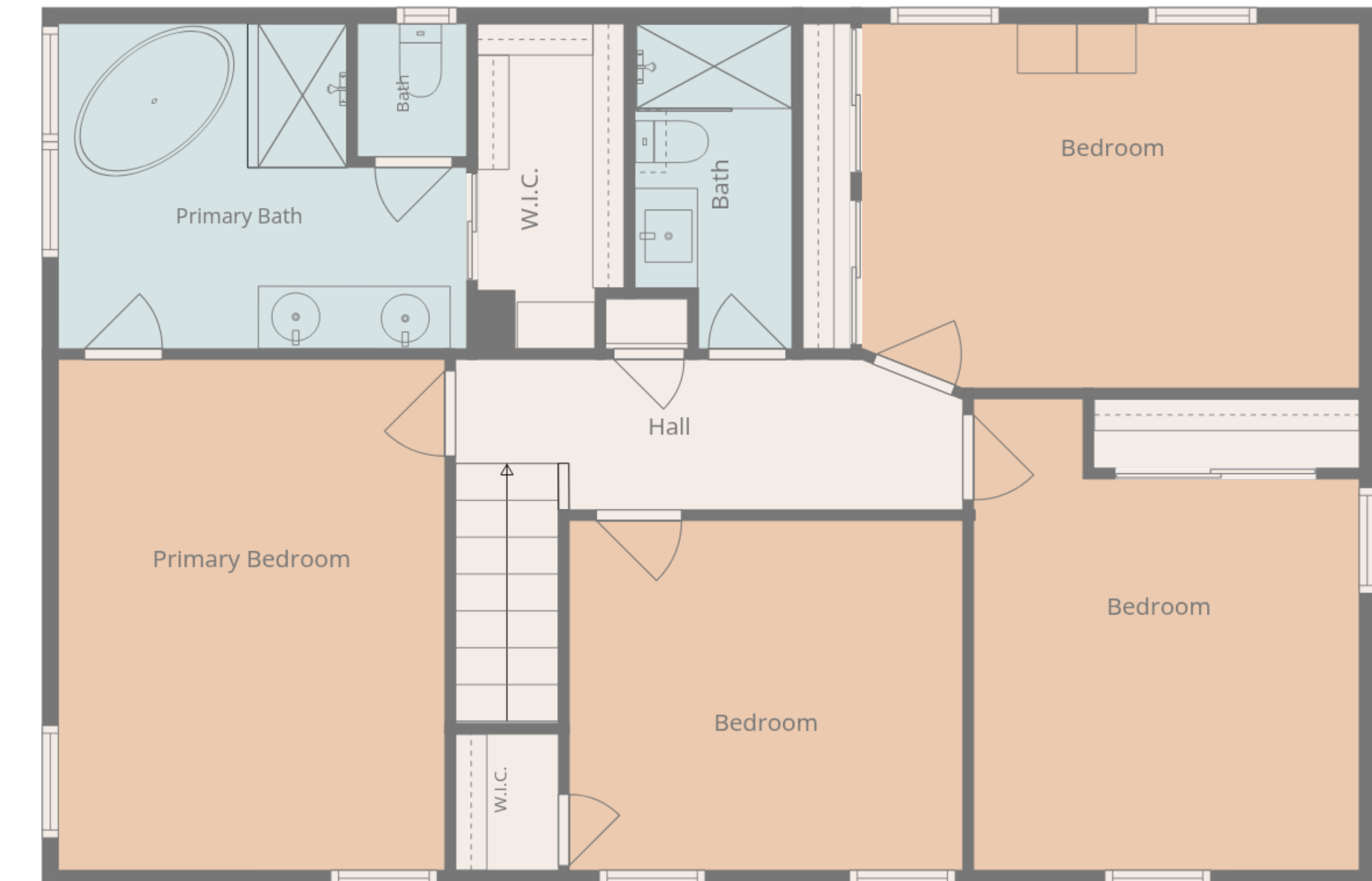
2nd Floor
