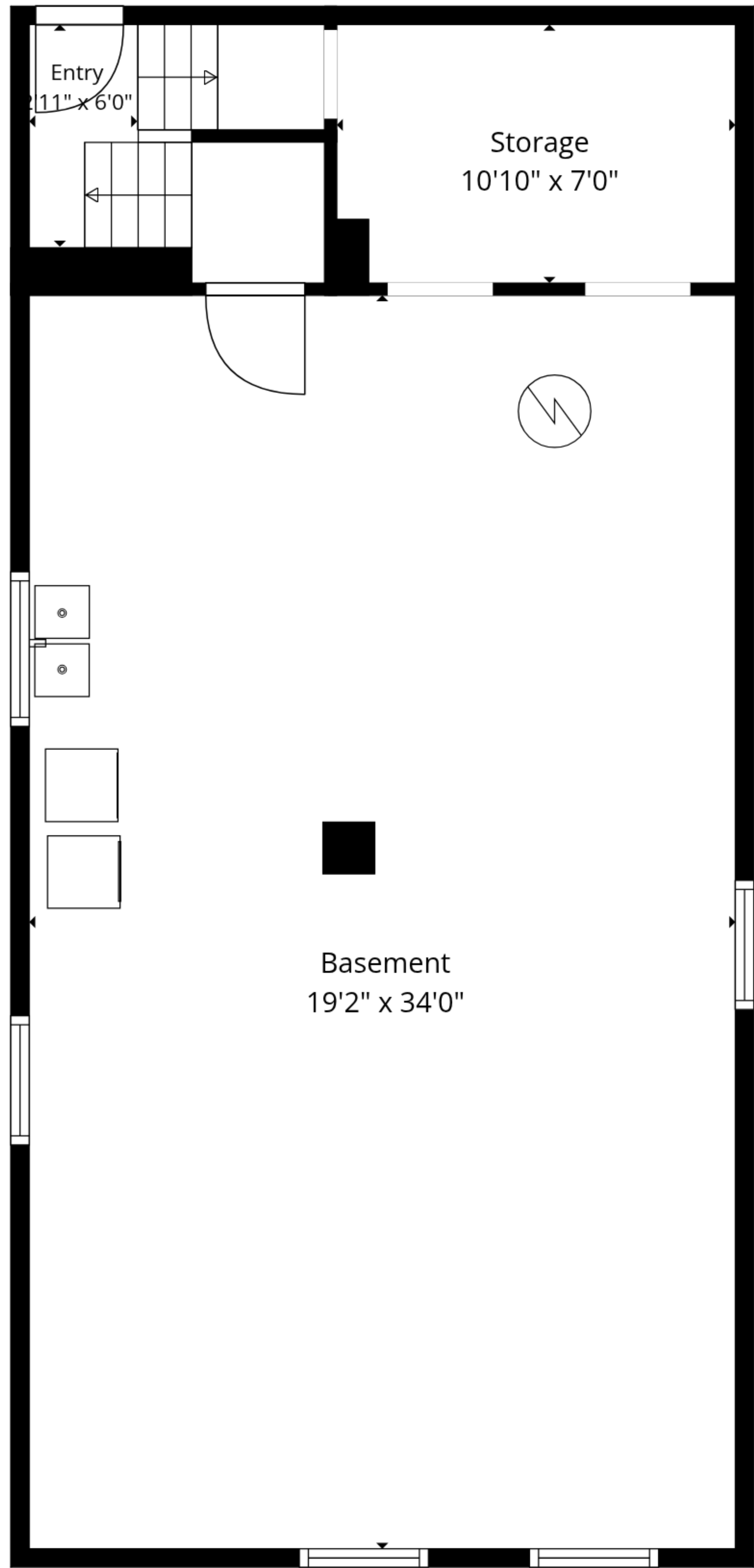
Basement
