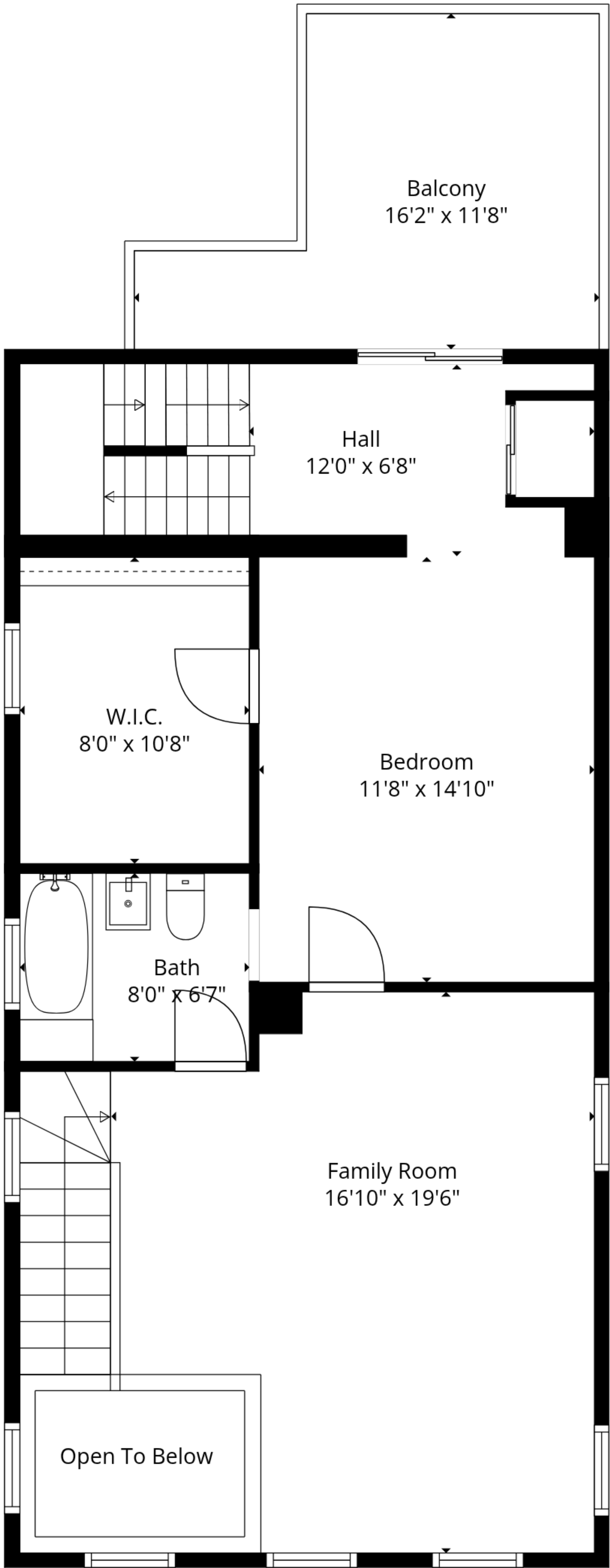
2nd Floor
